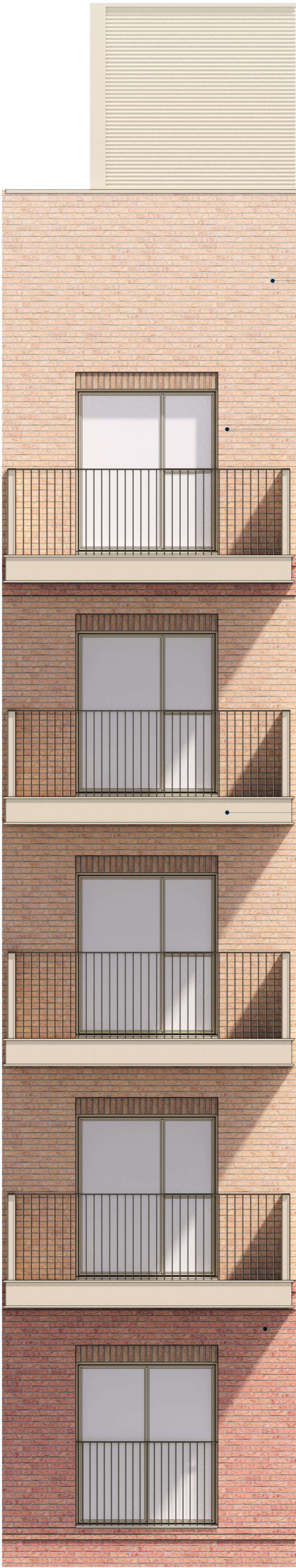
Elevation - C Bay Elevation 05 Lower
