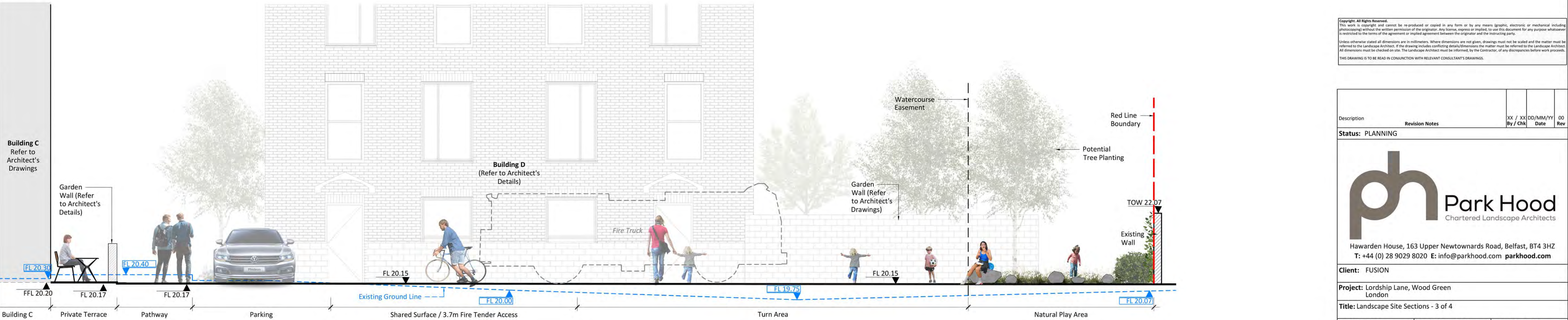
07 SECTION F-F Section Scale 1:50
