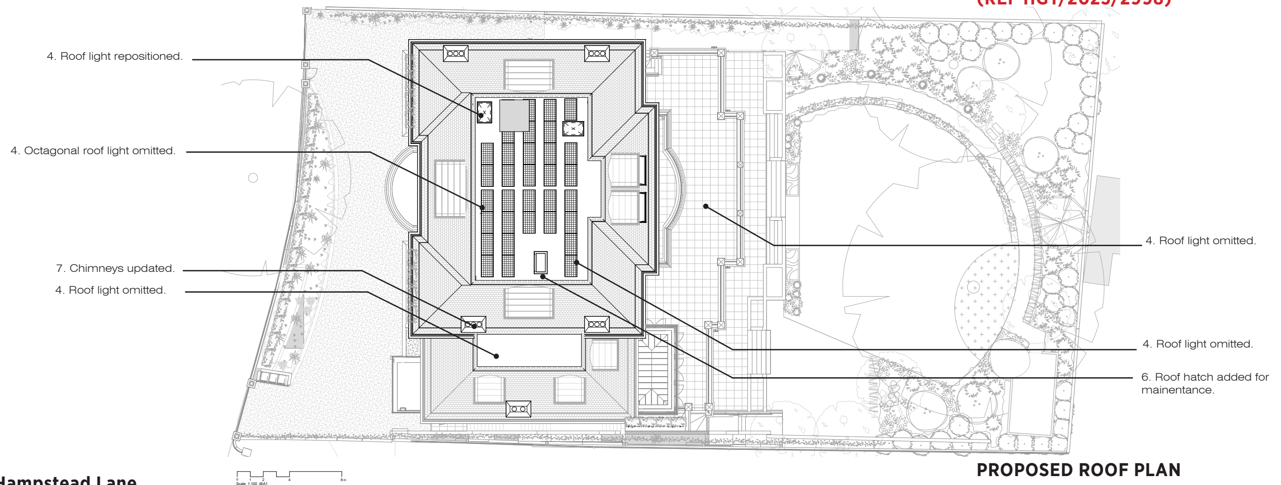
CONSENTED ROOF PLAN (REF HGY/2023/2998)
