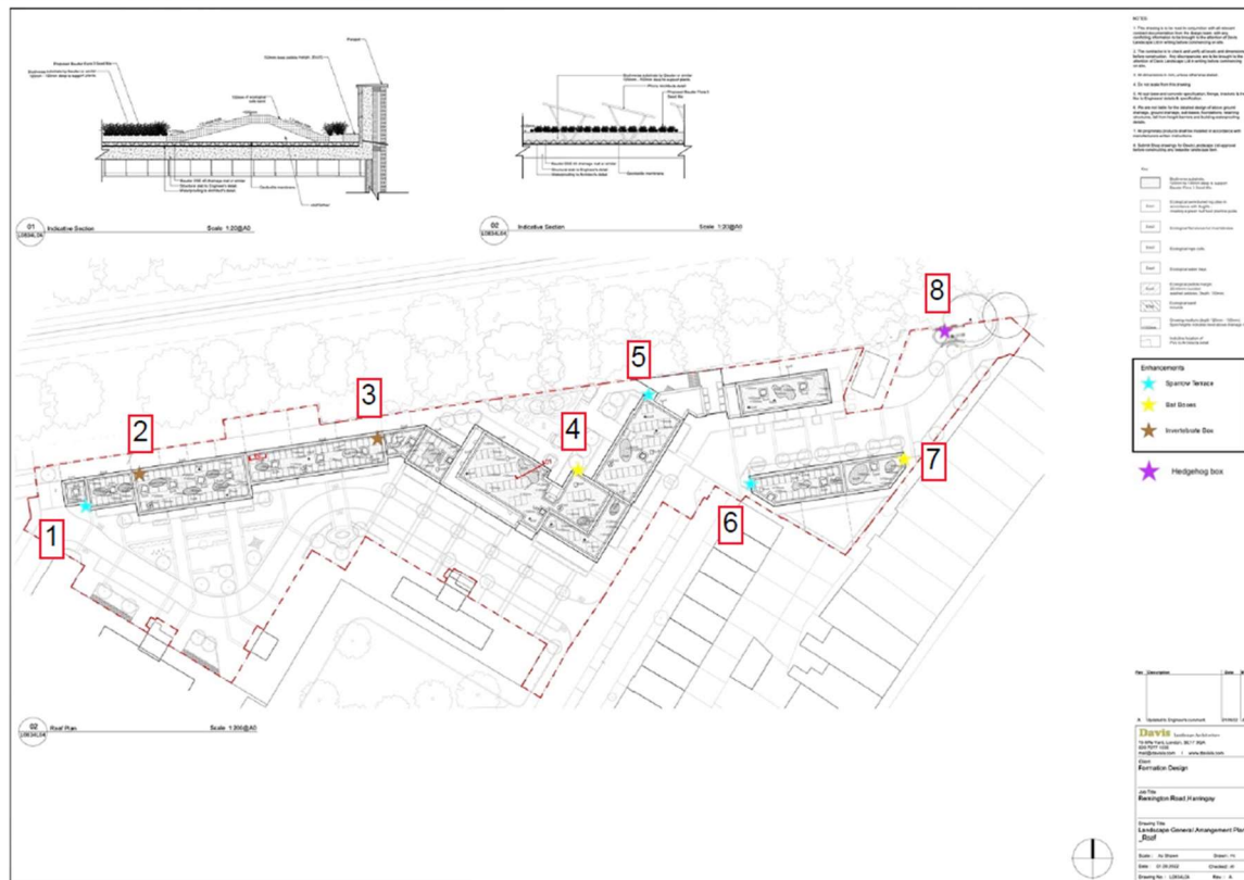
Figure 1: Roof plan with enhancement locations
