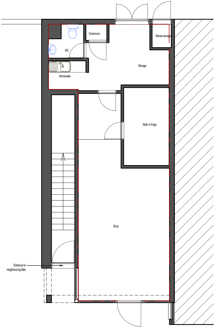
scale 1:100 0m 1m 2m 3m 4m 5m Ground Floor Plan - Existing
