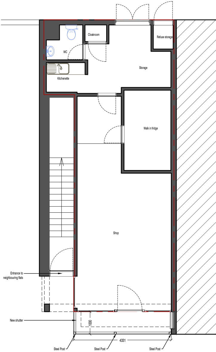
scale 1:100 0m 1m 2m 3m 4m 5m Ground Floor Plan - Proposed
