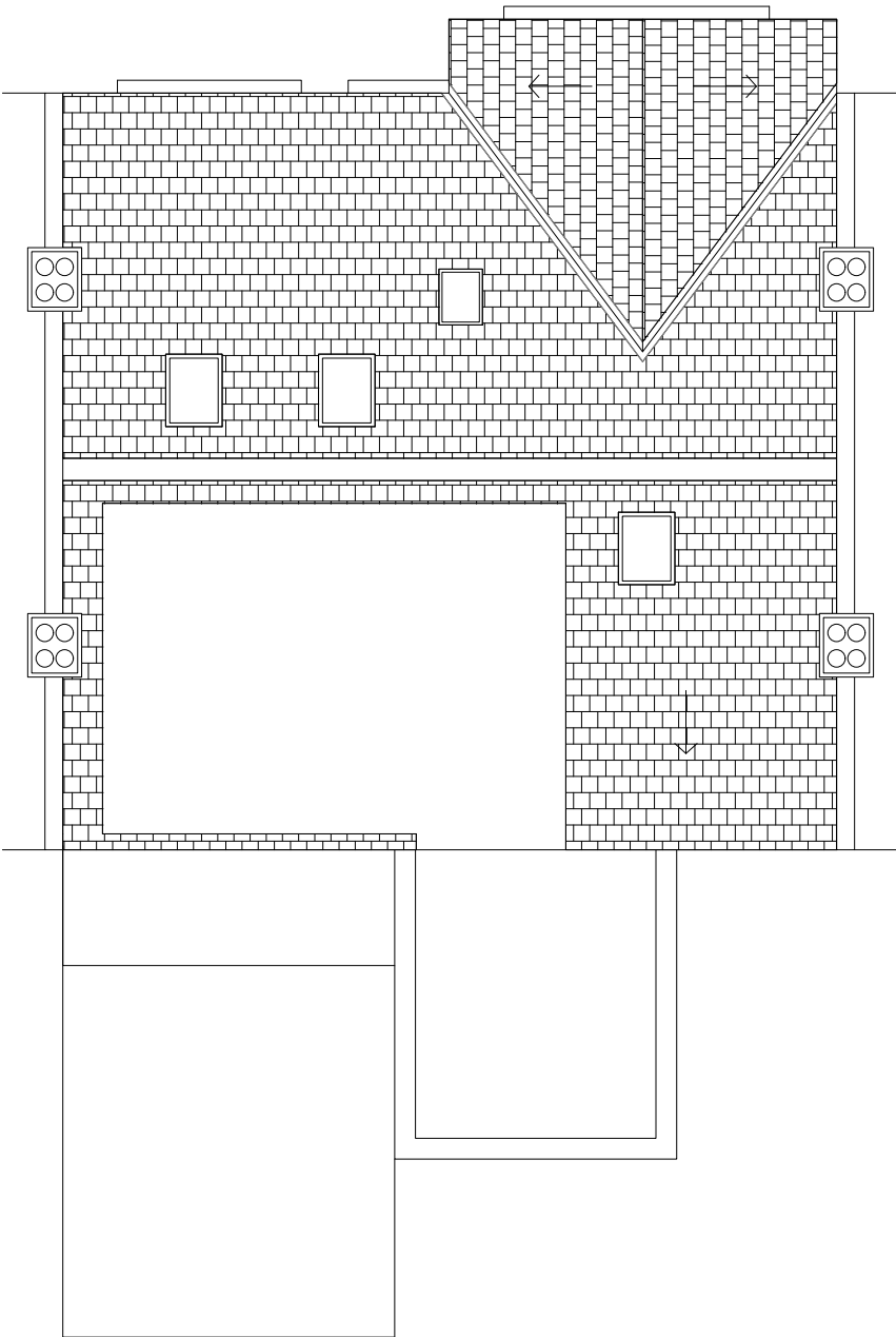
ROOF PLAN
