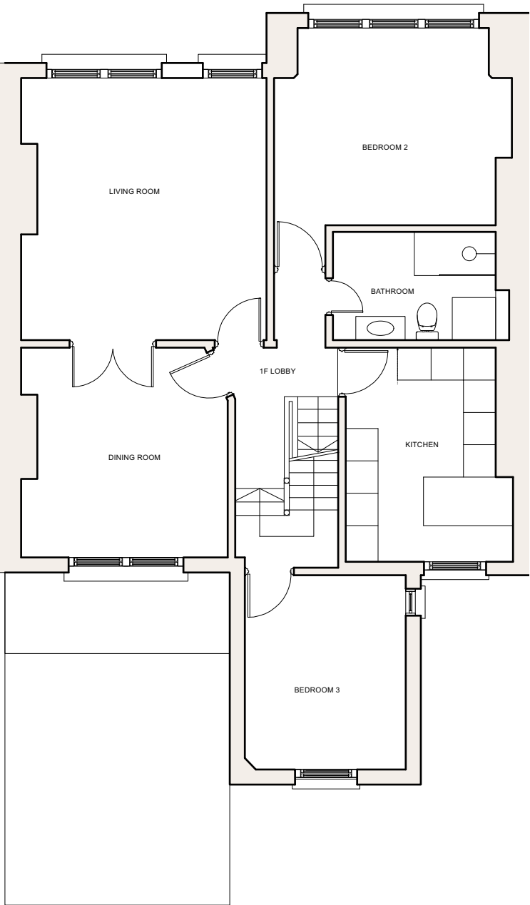
1F PLAN
