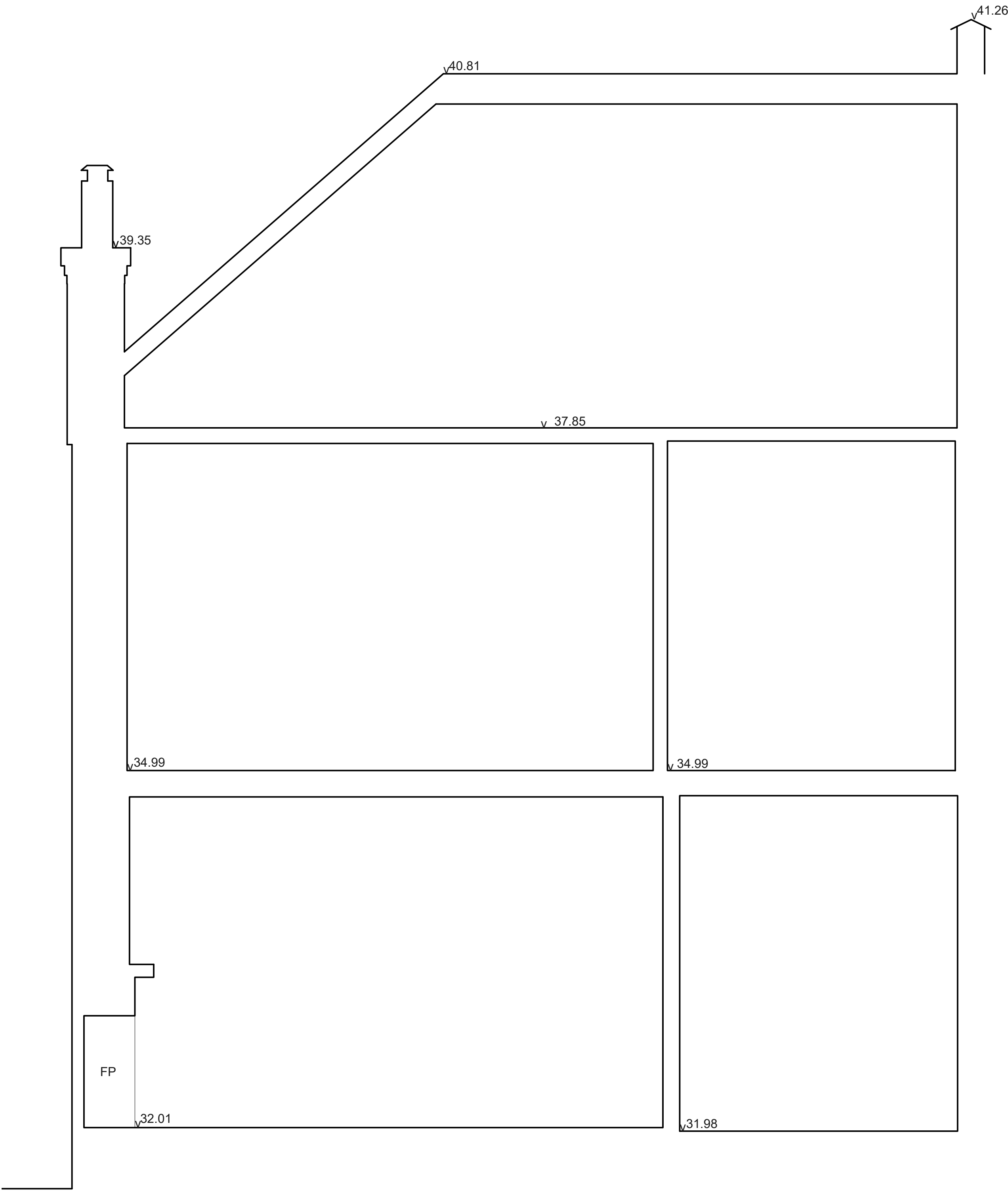
01 Section CC 1:25 @ A1
