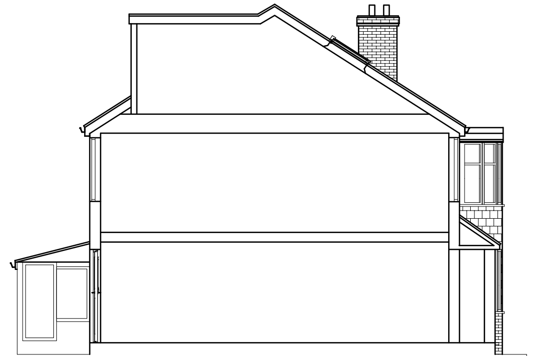
EXISTING SECTION
