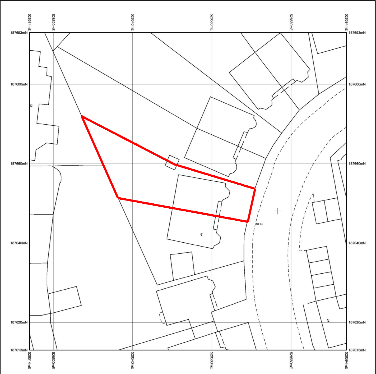
Block Plan 1:500
