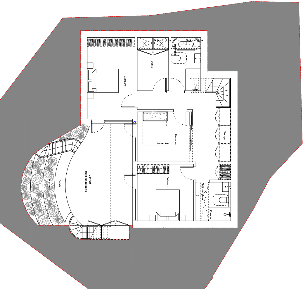
Proposed Lower Ground Floor
