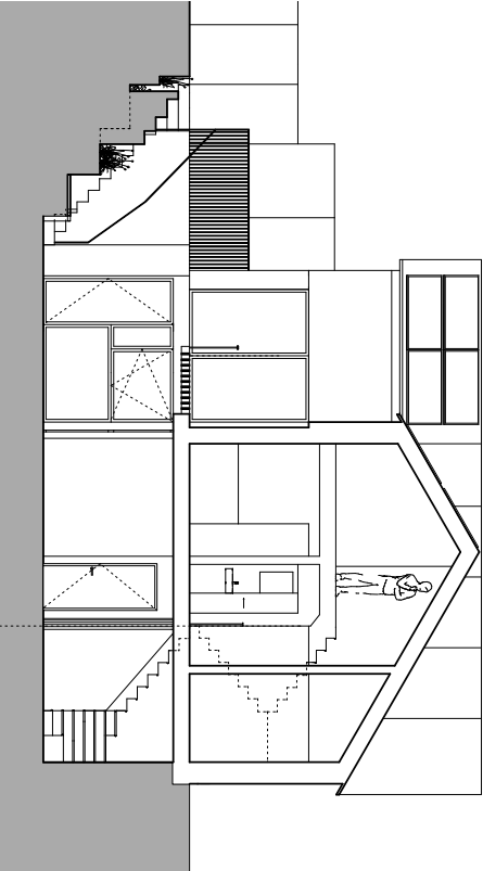
Proposed Section B
