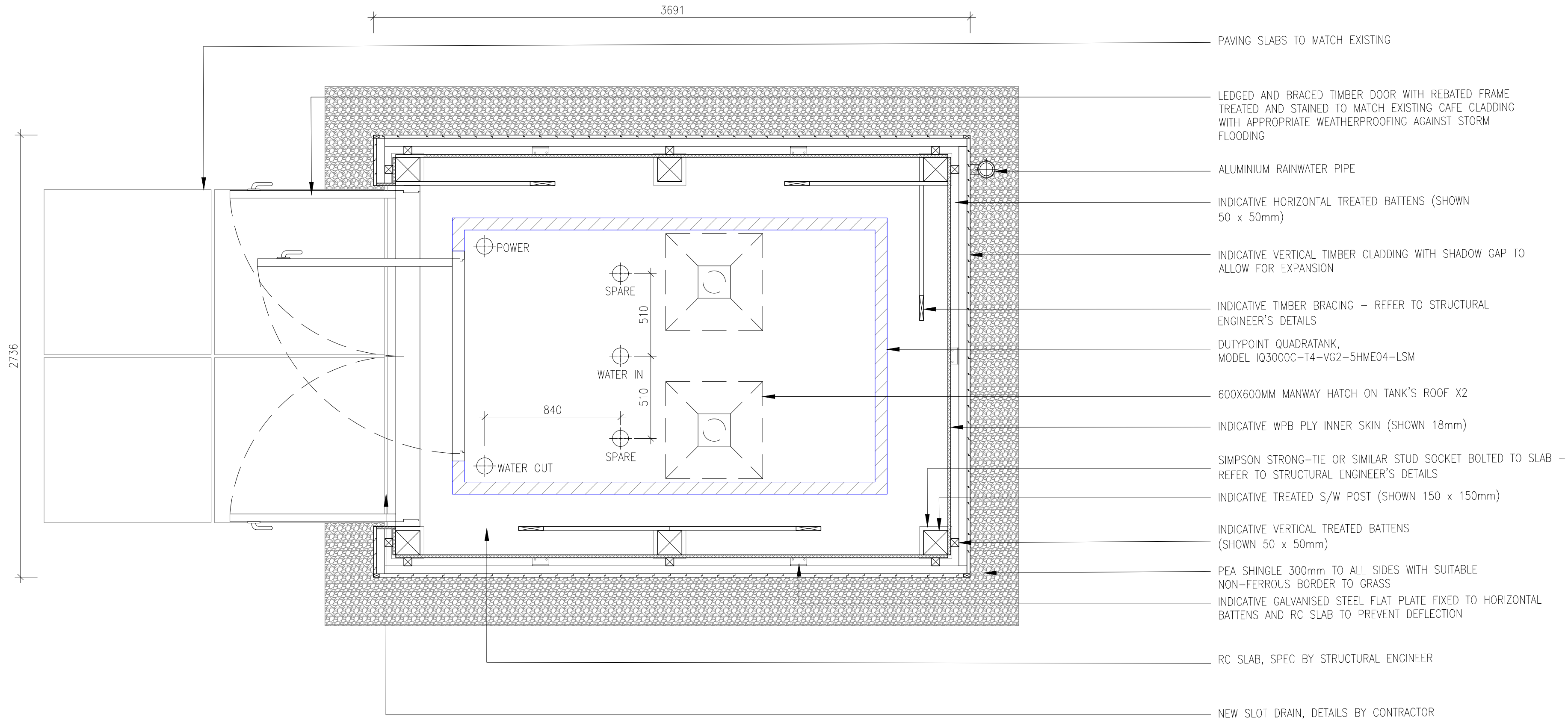
WATER TANK ENCLOSURE PLAN 0 2 METRES PRE-ASSEMBLED WATER TANK
