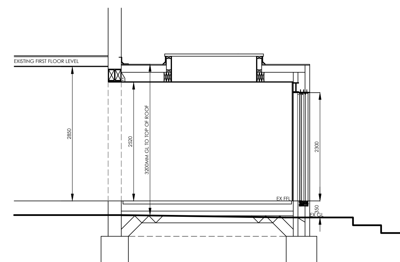
PROPOSED SECTION 1:50
