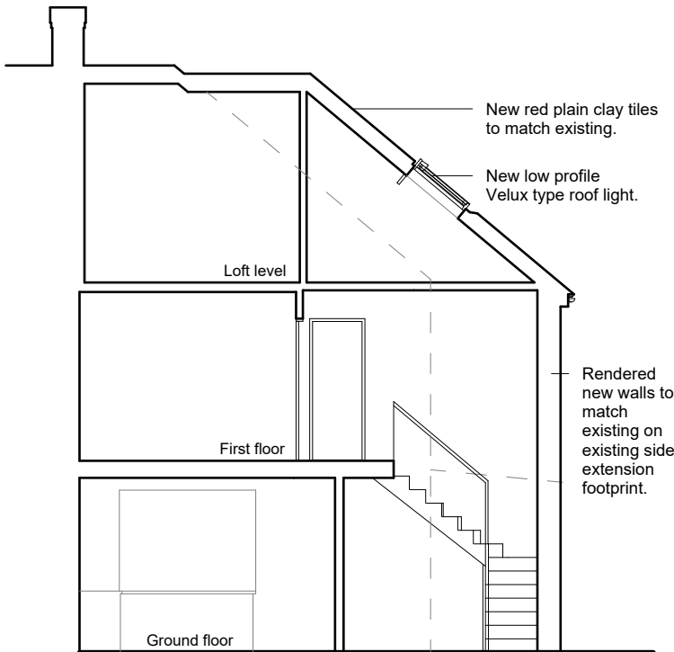
04 - Section A-A - proposed
