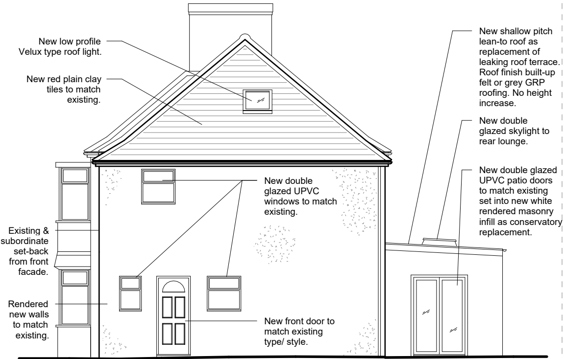
02 - Side elevation - proposed
