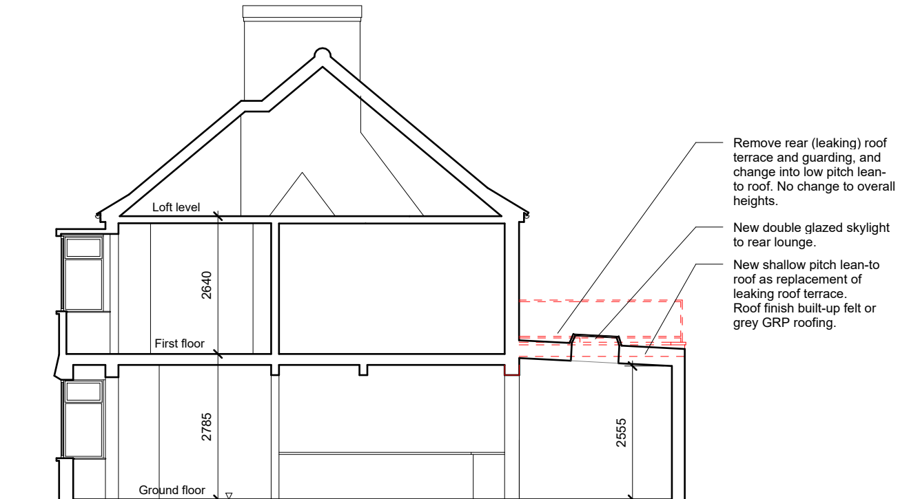
05 - Section B-B - proposed
