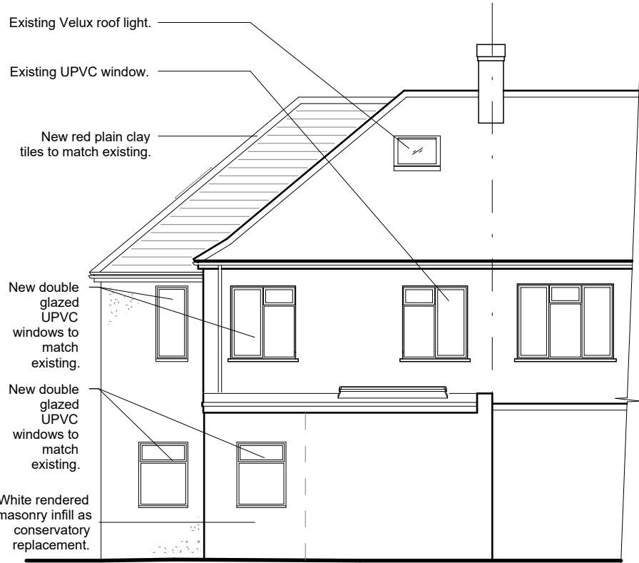
03 - Rear elevation - proposed
