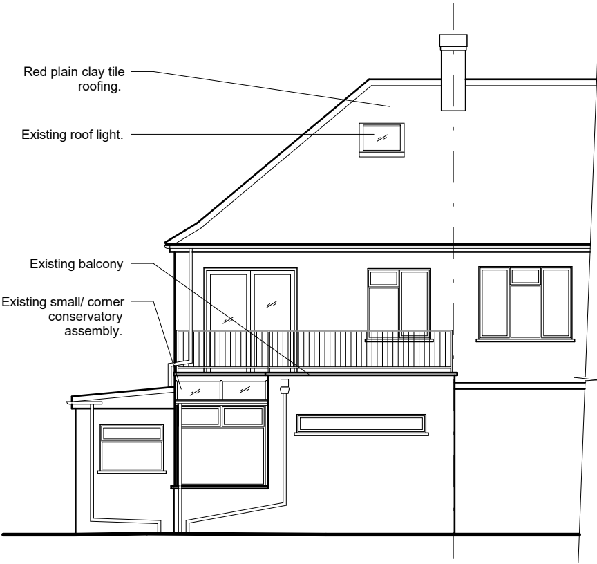
03 - Rear elevation - existing
