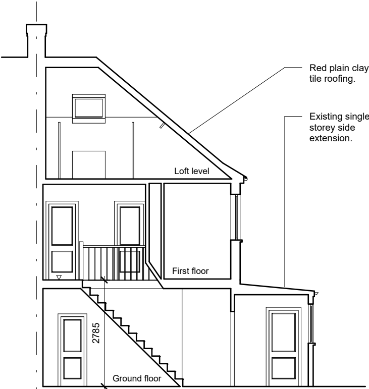
04 - Section A-A - existing
