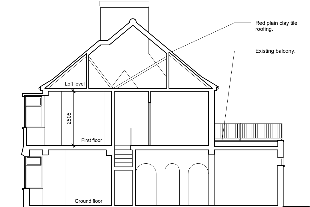
05 - Section B-B - existing
