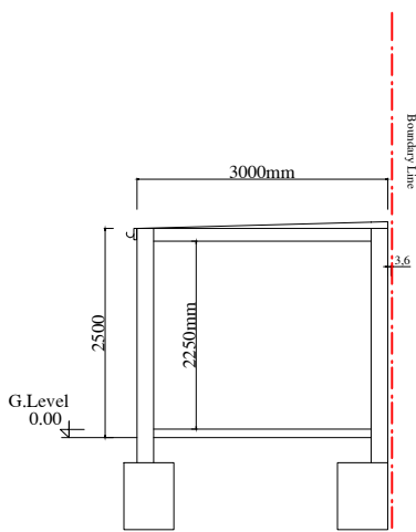
EXISTING SECTION A-A
