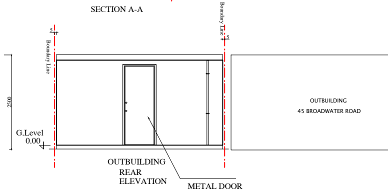
EXISTING SECTION A-A
