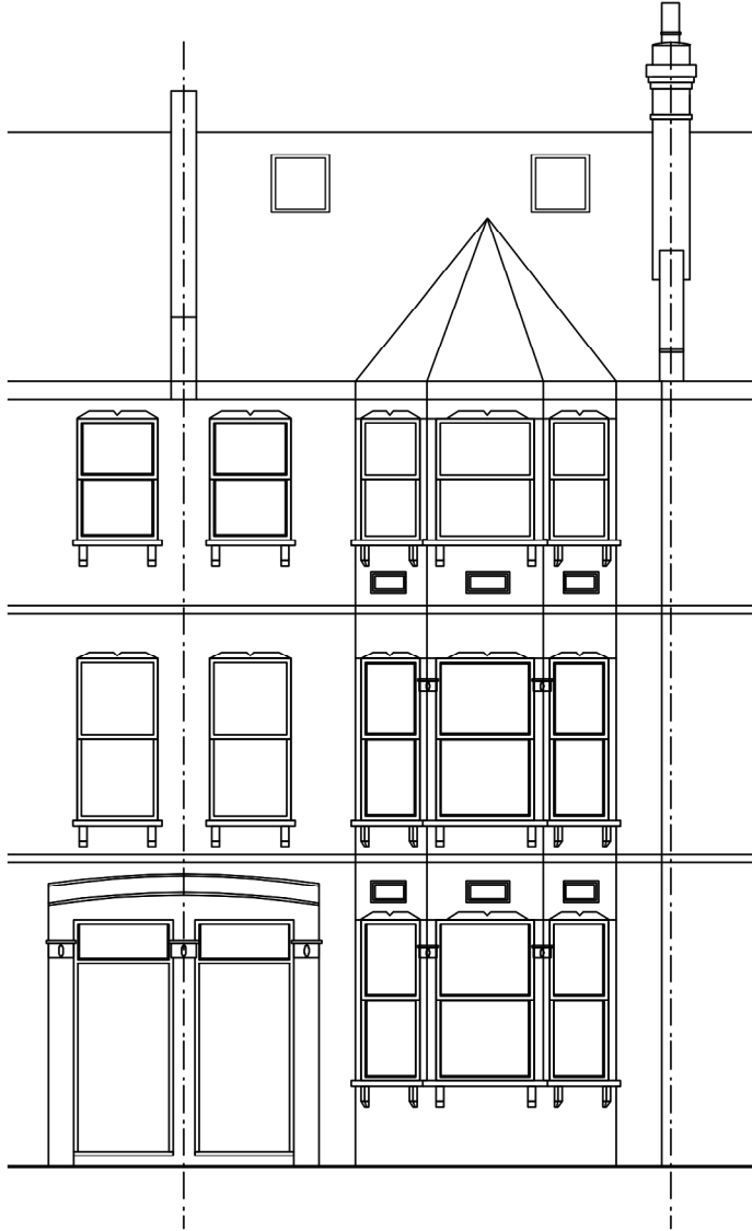
Front Elevation
