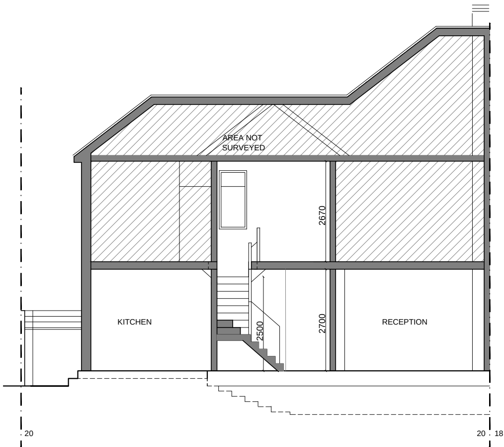
SECTION AA
