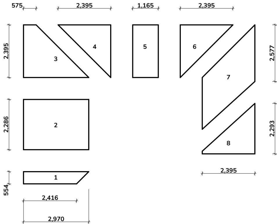
Simplified & Exploded Roof Additional Volume Plan Split in to calculable prisms
