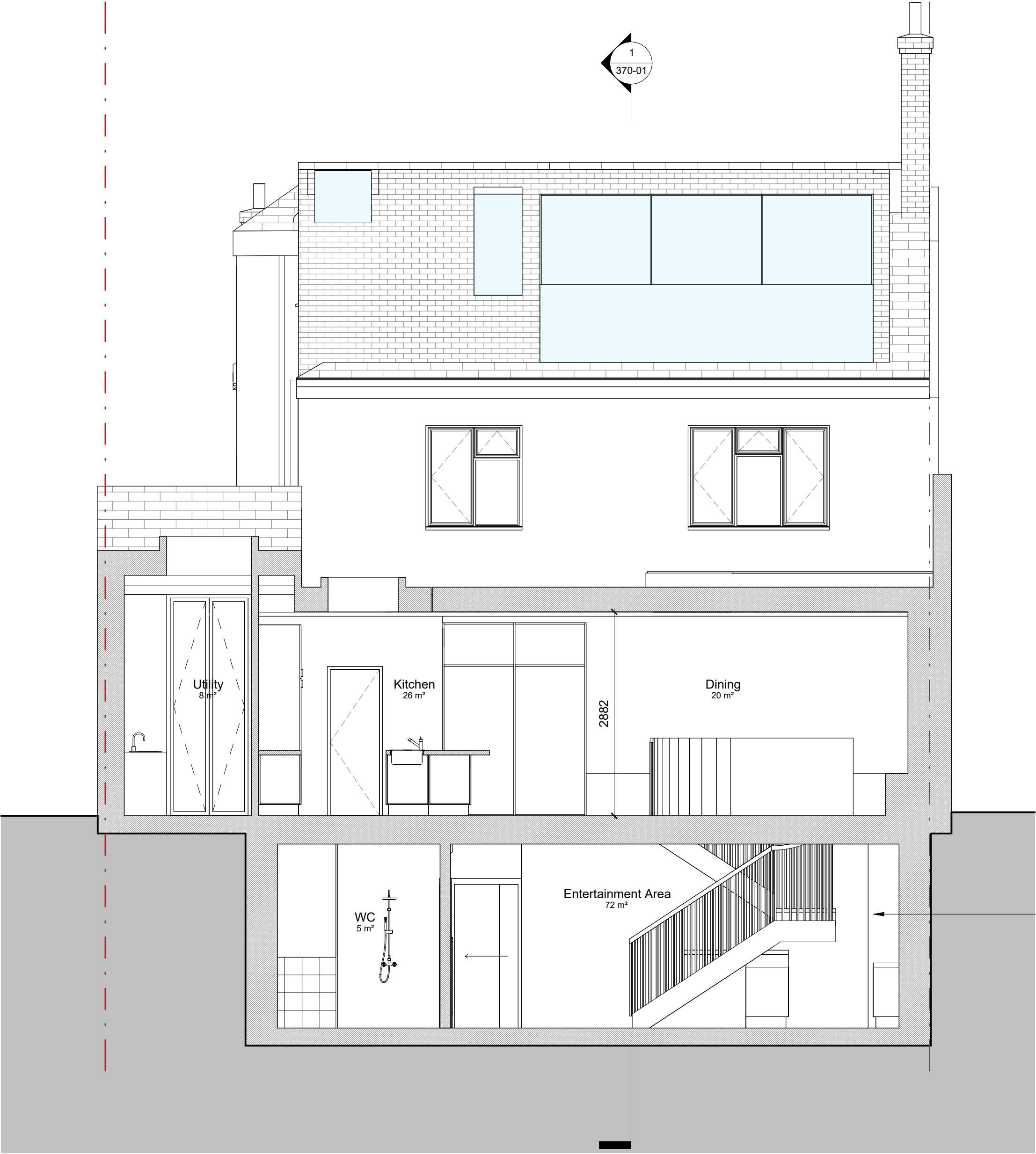
2 Proposed Cross Section 1 : 50
