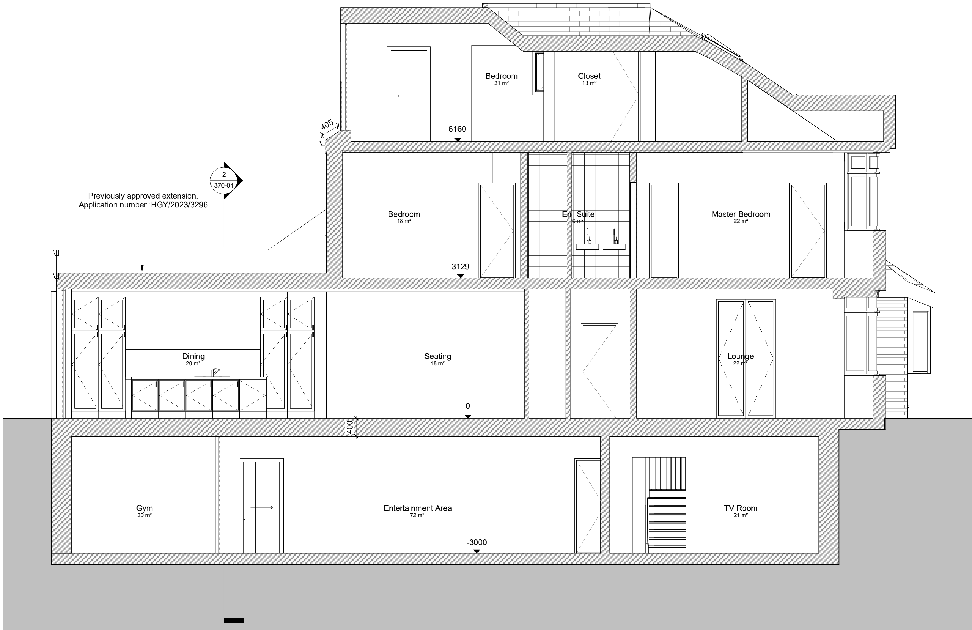
1 Proposed Long Section 1 : 50
