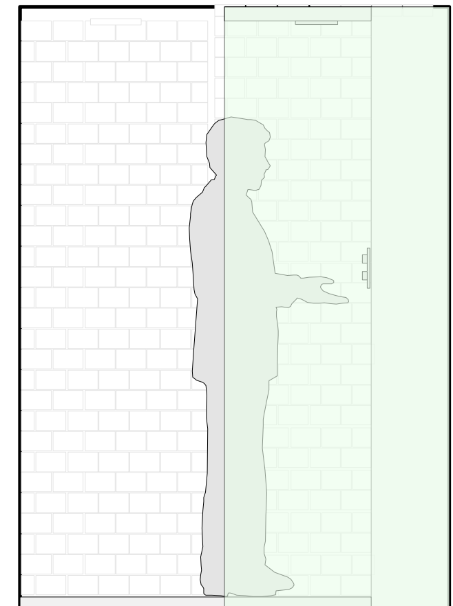
section through shower showing floor to ceiling fixed glass screen scale 1:20
