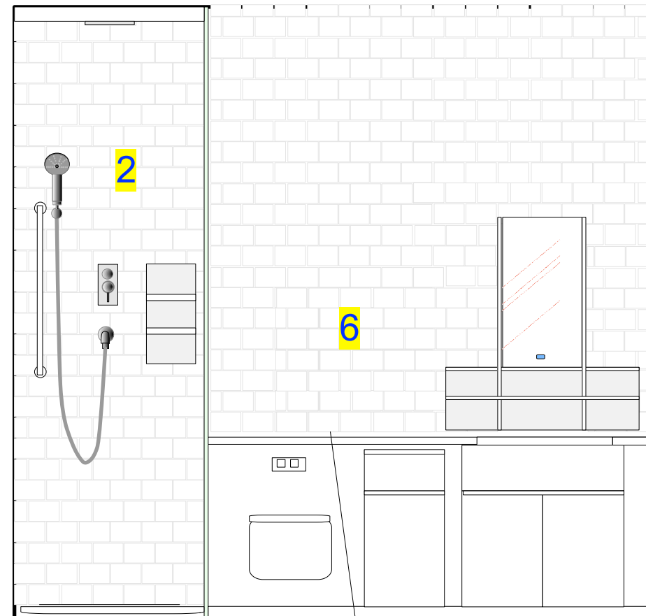
section through bathroom scale 1:20
