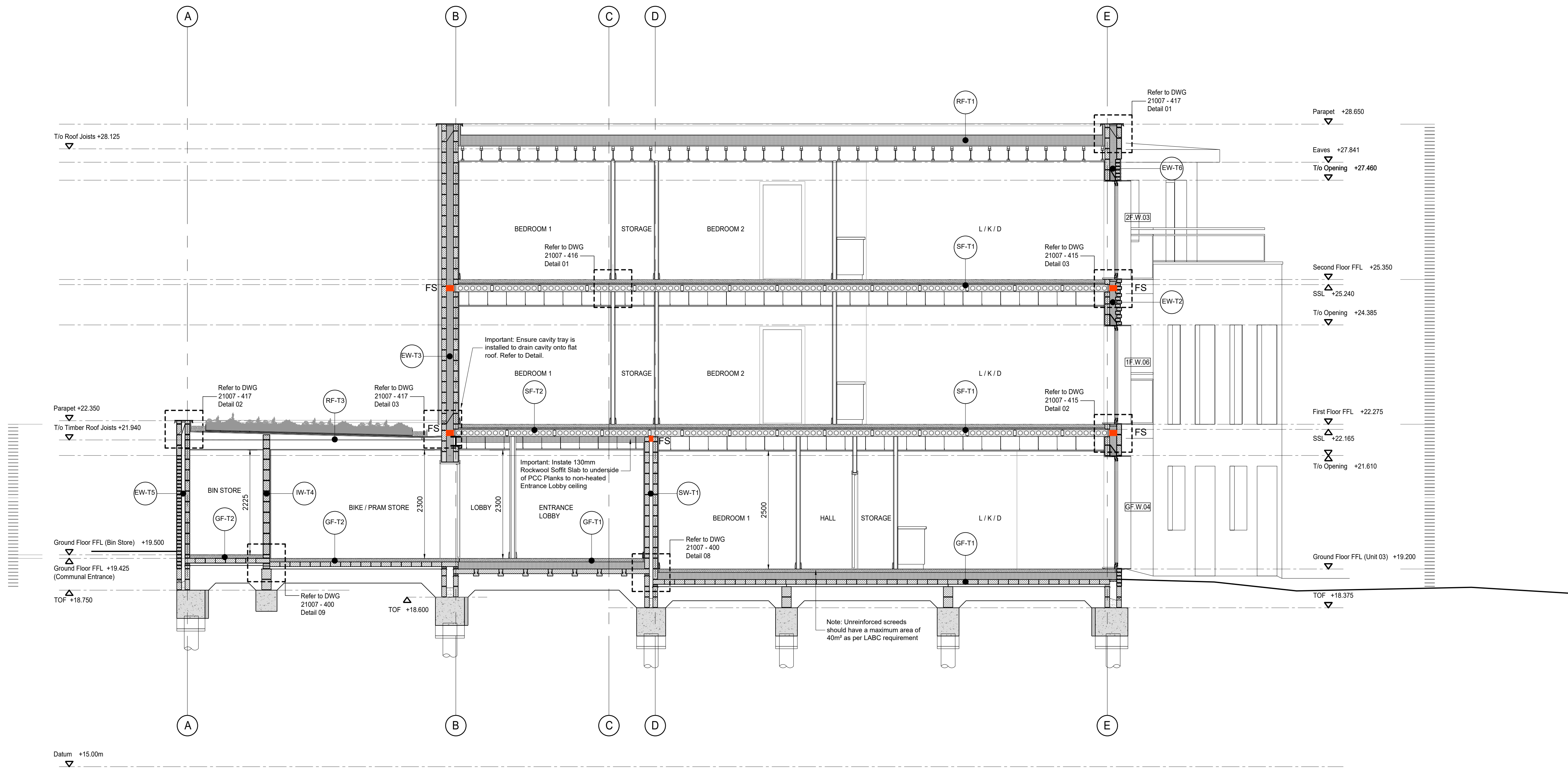
Section B-B
