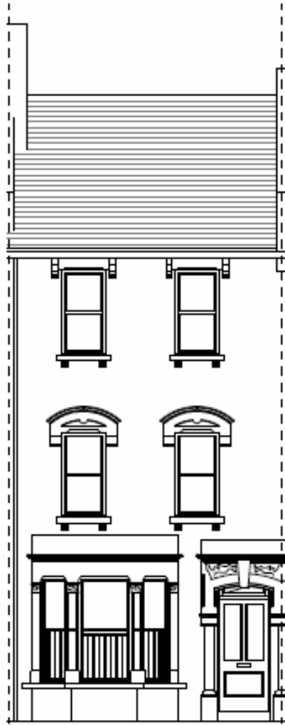
Existing Ground Floor Front Elevation
