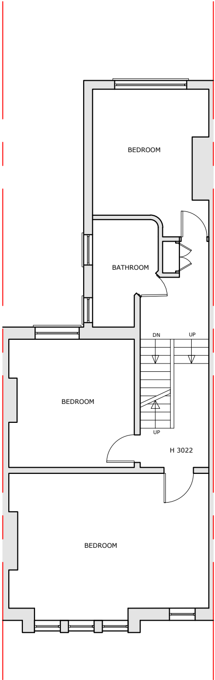
PROPOSED FIRST FLOOR PLAN SCALE 1:100 - UNCHANGED
