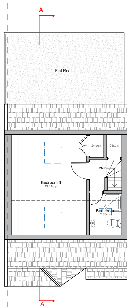
EXISTING LOFT PLAN
