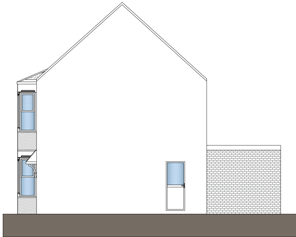
EXISTING SOUTH EAST ELEVATION
