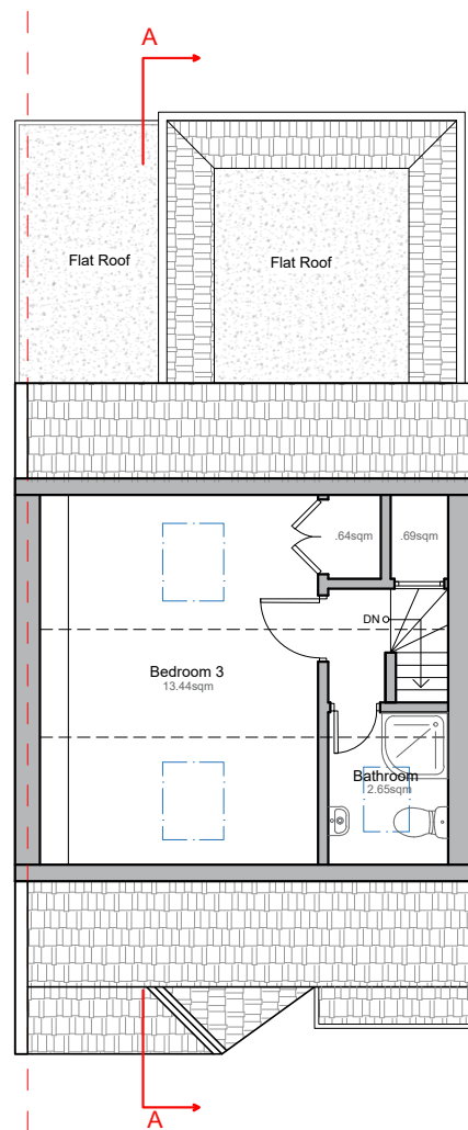
PROPOSED LOFT PLAN
