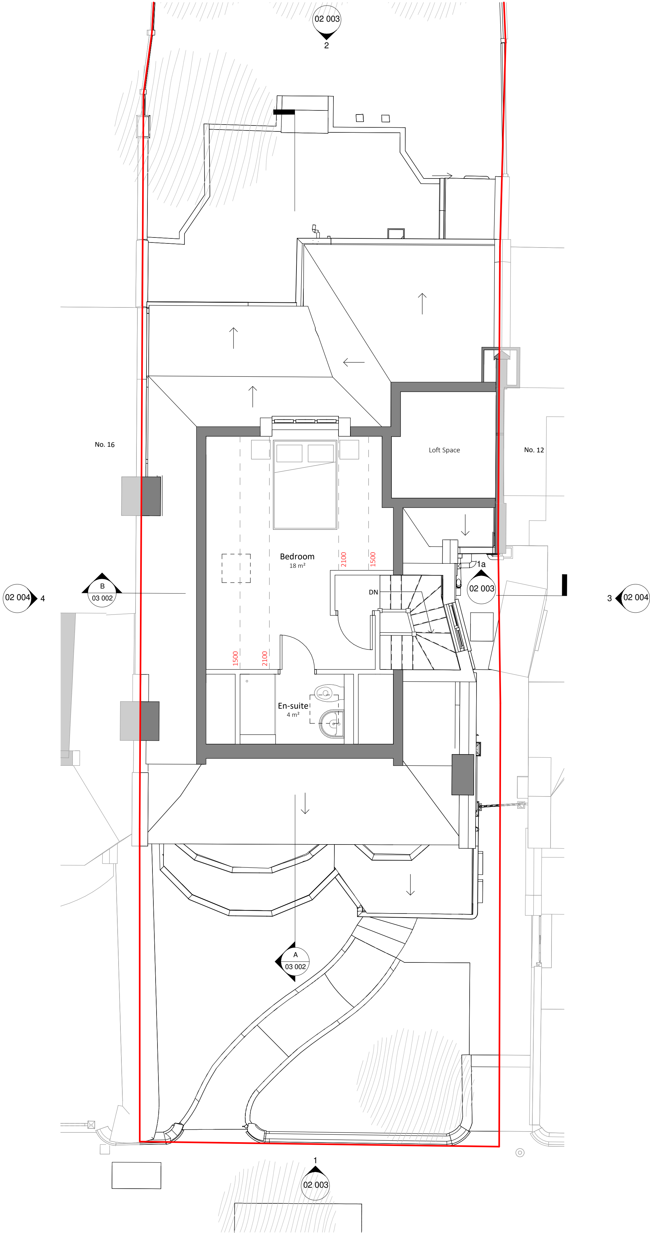
2 Level 02 Proposed 1 : 50
