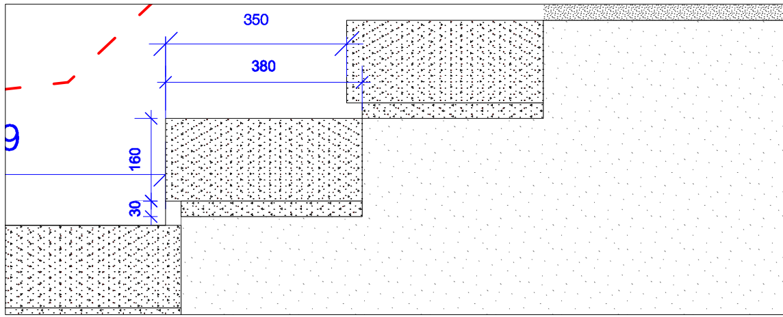
Step Detail
