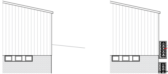
PROPOSED FRONT ELEVATION A 1:100@ A3
