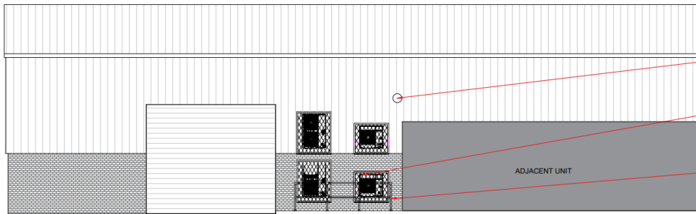
PROPOSED FRONT ELEVATION A 1:100@ A3
