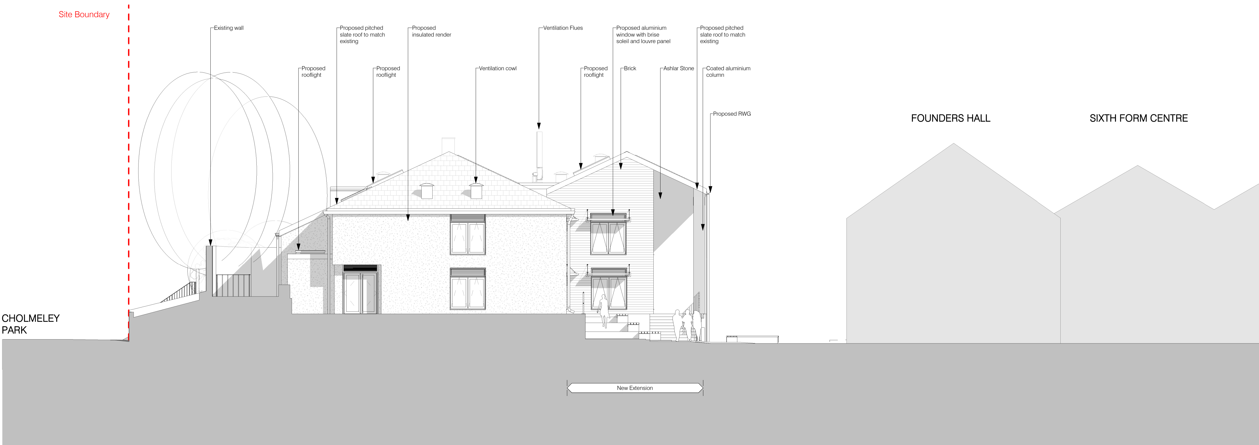
Proposed - Elevation B 1 : 100
