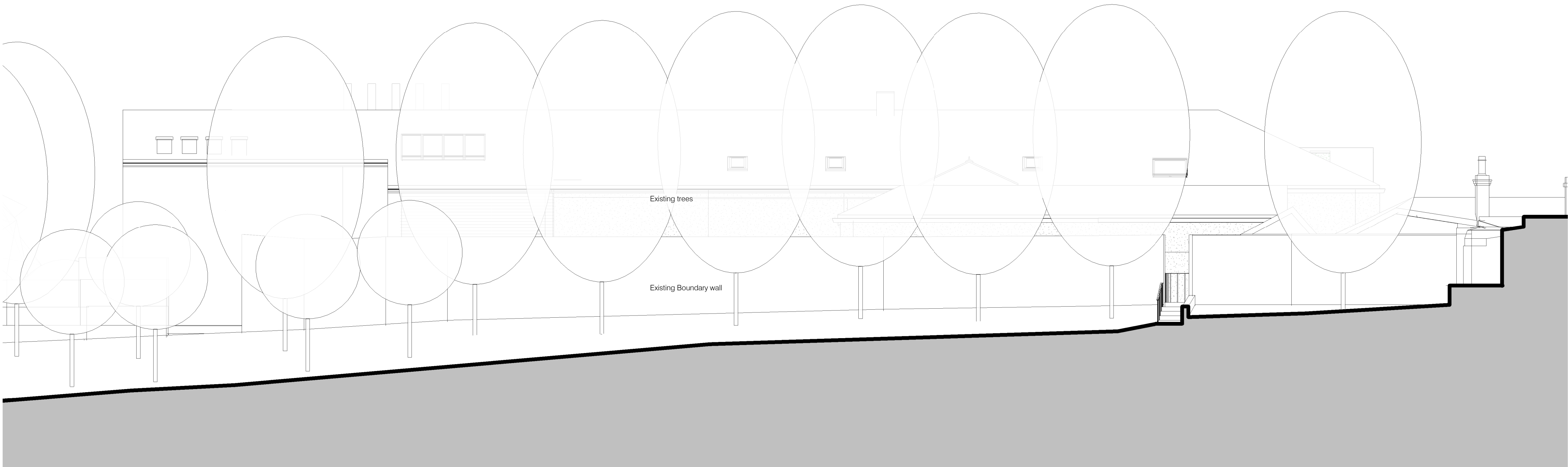
Proposed Northwest Elevation 1:100
