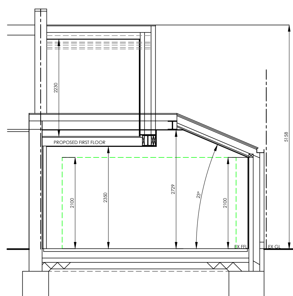
PROPOSED SECTION 1:50
