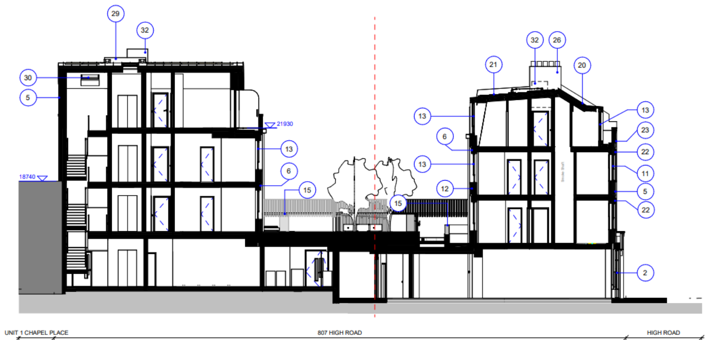
Proposed section – Block A (fronting High Road) on right and Block B on the left
