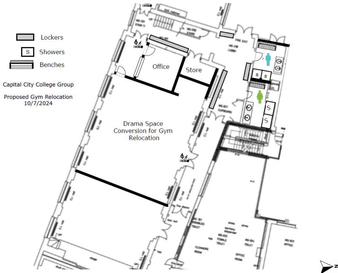
Figure 2: Layout of gym/showers/lockers
