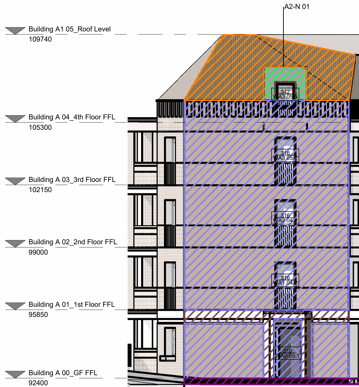
Block A2 - North Elevation 1 : 100
