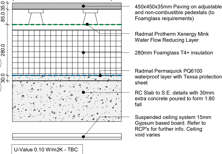
ROOF TYPE R5: INSULATED BALCONY BUILDING A (GF LEVEL ABOVE RESIDENTIAL UNITS)
