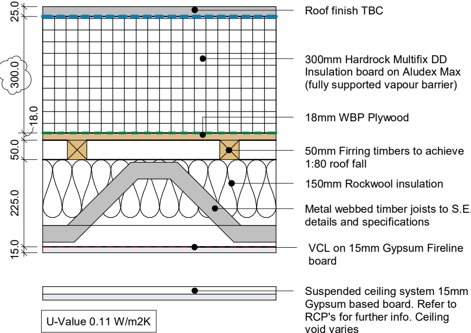
ROOF TYPE R3: FLAT ROOF BUILDING C
