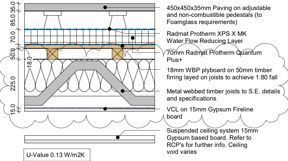
ROOF TYPE R4: PAVED ROOF (TERRACE) BUILDING C
