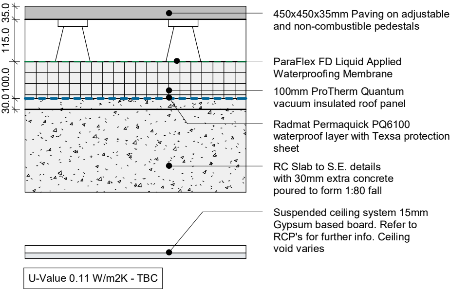
ROOF TYPE R2: PAVED ROOF (TERRACE) BUILDINGS A&B
