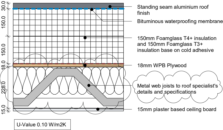
ROOF TYPE R1: SLOPING (MANSARD) ALUMINIUM ROOF
