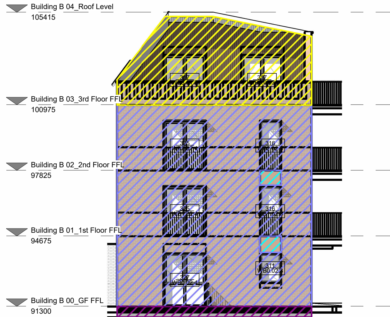
Block B - South Elevation 1 : 100
