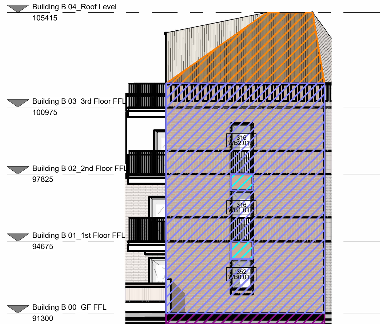
Block B - North Elevation 1 : 100
