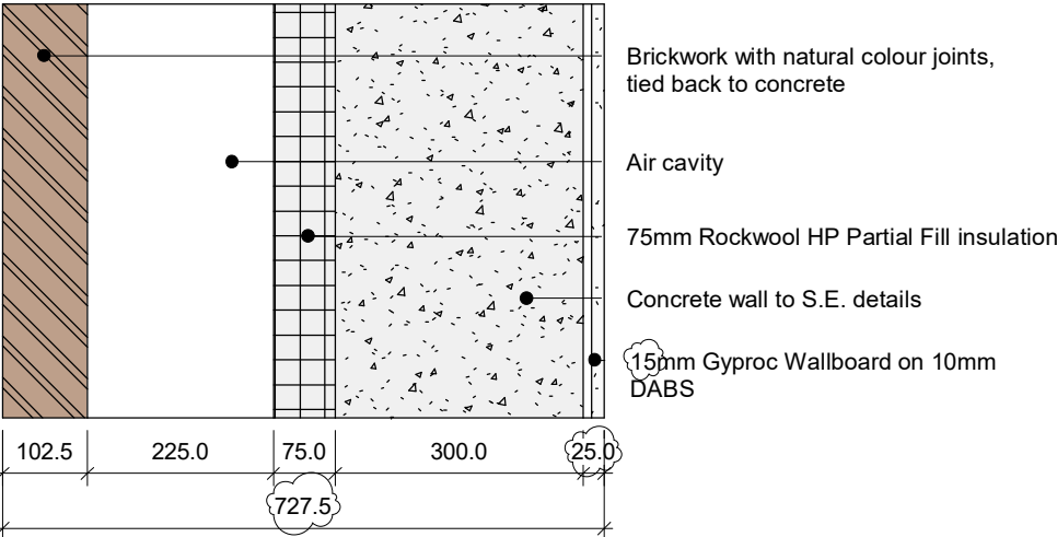
TYPE E9: BRICK AND CONCRETE WALL TO BUILDING A CYCLE STORE (LOWER GROUND FLOOR LEVEL)
