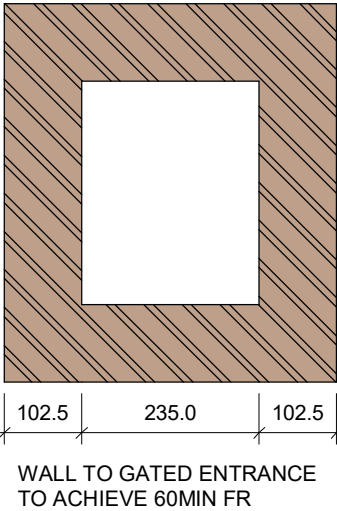
TYPE E10: BRICK WALL AT BUILDING COMMUNAL CORRIDOR TYPE E10B: CERAMIC WALL AT BUILDING A GATED ENTRANCE
