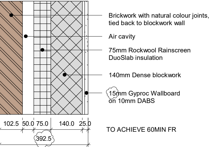
TYPE E7: BRICK WALL TO ANCILLARY AREAS ANS STAIRS BUILDING A
