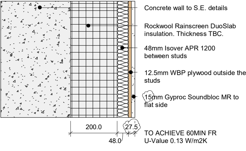
TYPE E8: CONCRETE WALL AGAINST TERRAIN TO BUILDING A RESIDENTIAL UNITS
