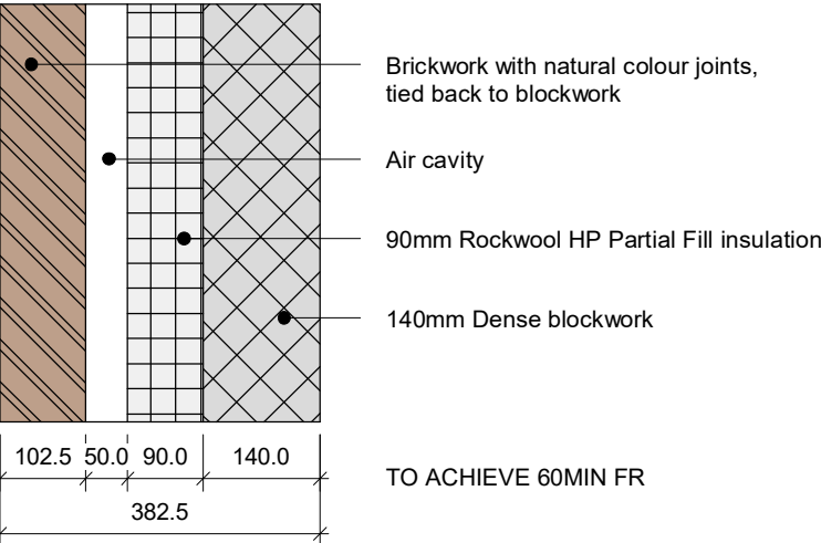
TYPE E9: BRICK AND CONCRETE WALL TO BUILDING A CYCLE STORE (LOWER GROUND FLOOR LEVEL)
