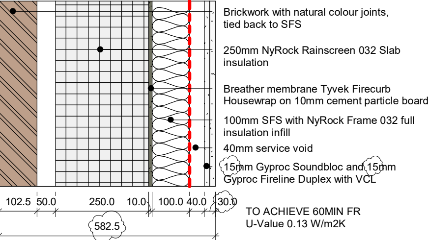
TYPE E4: STAIR EXTERNAL WALL BUILDING B TYPE E4B: VERTICAL STACK BOND (SOLDIER) STAIR EXTERNAL WALL BUILDING B TYPE E4C: CERAMIC FINISH STAIR EXTERNAL WALL BUILDING B
