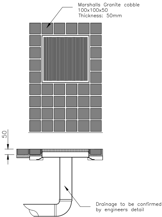
Detail 05 1:20 – Planter Passage
