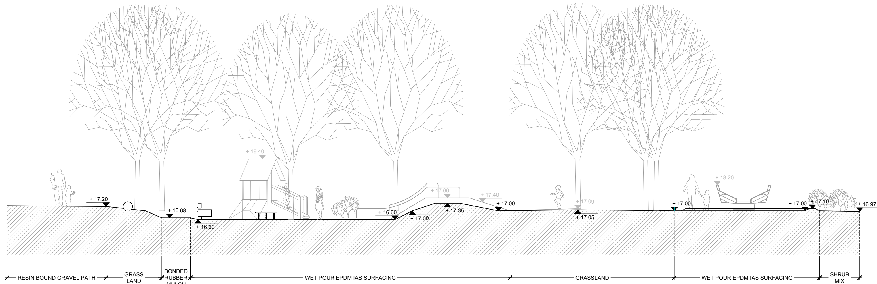
PLAY AREA SECTION SCALE 1:100 @ A1
