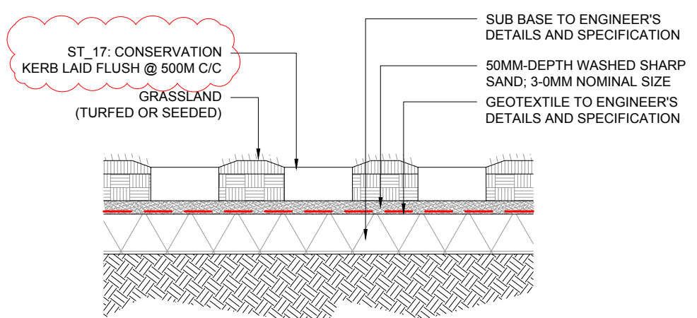
04 CONCRETE KERB & TURF INTERFACE TYPICAL SECTION - 1:20 @ A1
