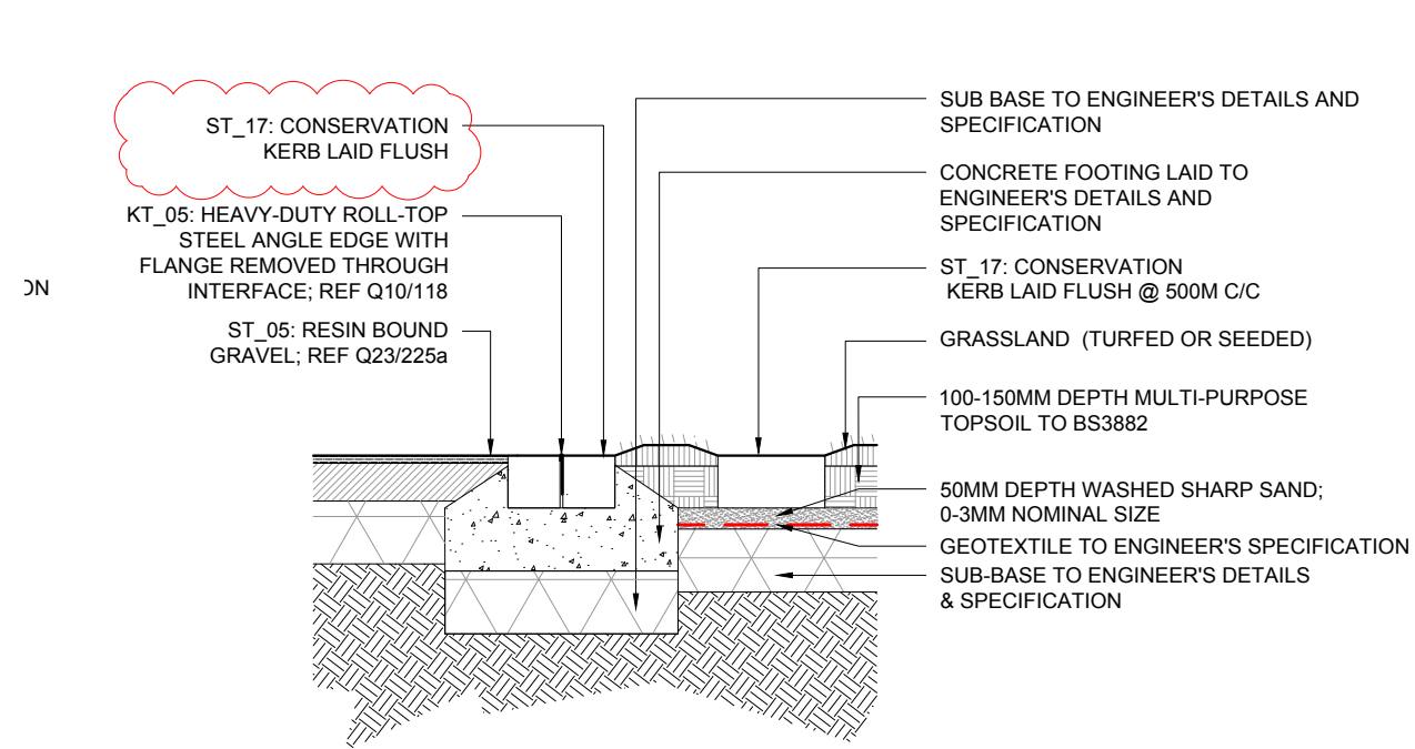
02 CONCRETE KERB & STEEL EDGE INTERFACE TYPICAL SECTION - 1:20 @ A1
