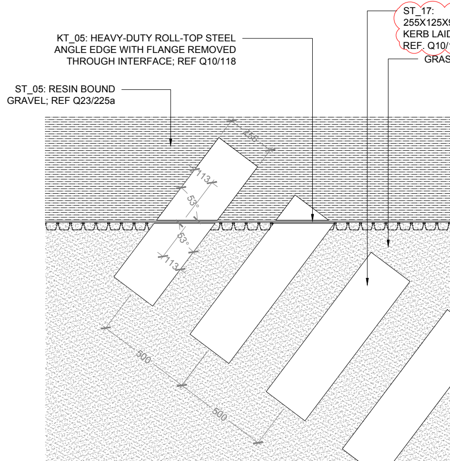
01 RESIN BOUND GRAVEL, STEEL EDGE & TURF INTERFACE TYPICAL PLAN - 1:20 @ A1
