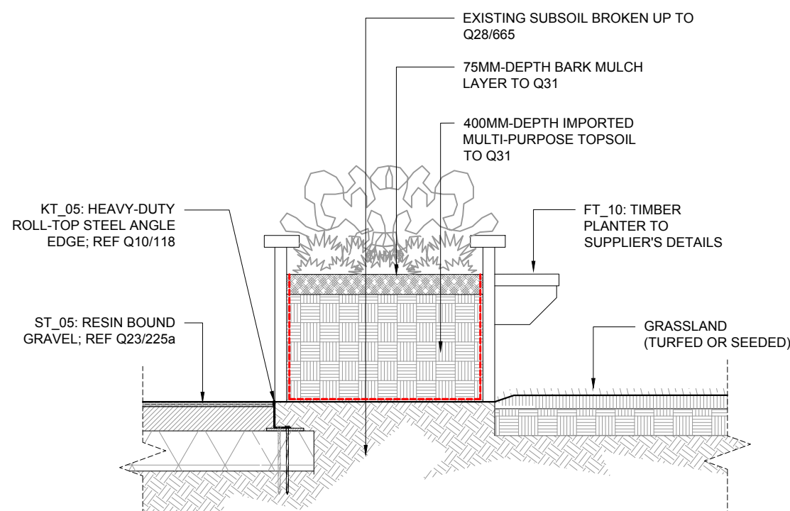
06 RESIN BOUND GRAVEL, STEEL EDGE, PLANTER & TURF INTERFACE TYPICAL SECTION - 1:20 @ A1
