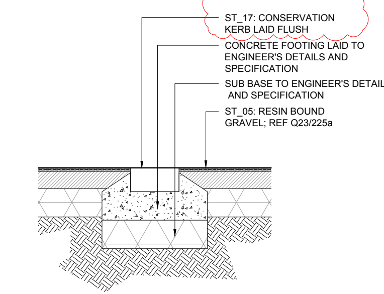
03 RESIN BOUND GRAVEL & CONCRETE KERB INTERFACE TYPICAL SECTION - 1:20 @ A1
