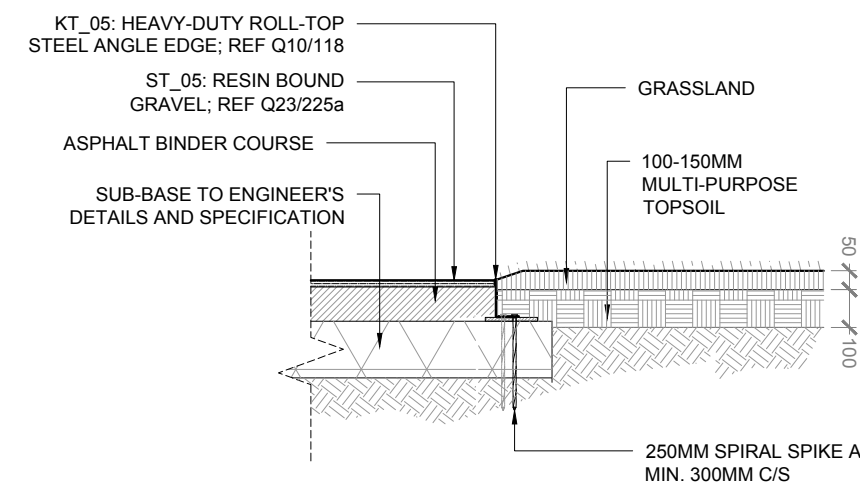
05 RESIN BOUND GRAVEL, STEEL EDGE & TURF INTERFACE TYPICAL SECTION - 1:20 @ A1
