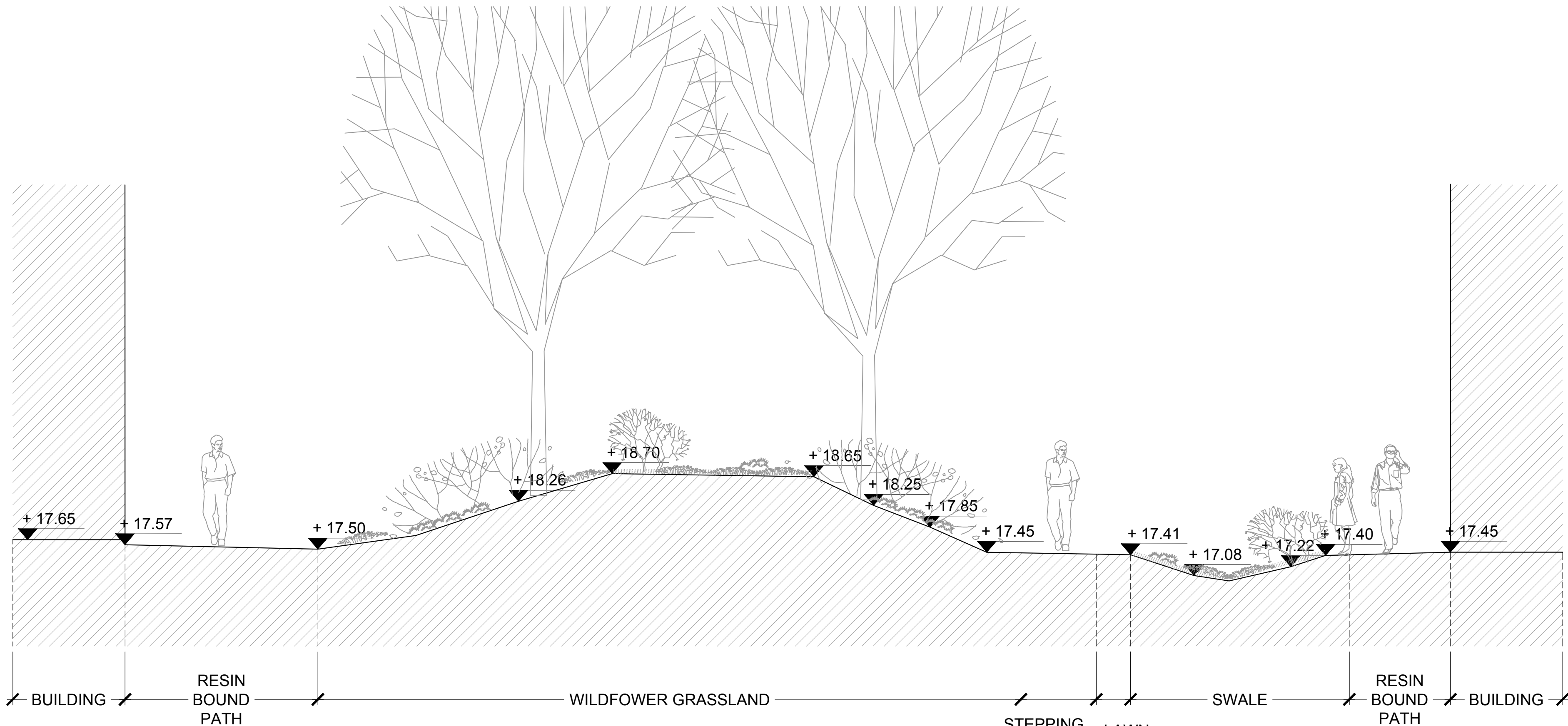
COURTYARD SECTION 1:50 @ A1
