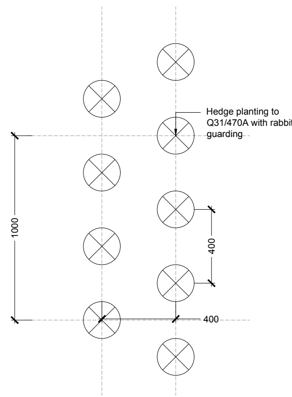
06 TYPICAL DOUBLE STAGGERED HEDGE PLANTING - REF S1
