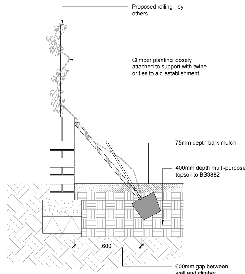
12 CLIMBING PLANTS - REF: C
