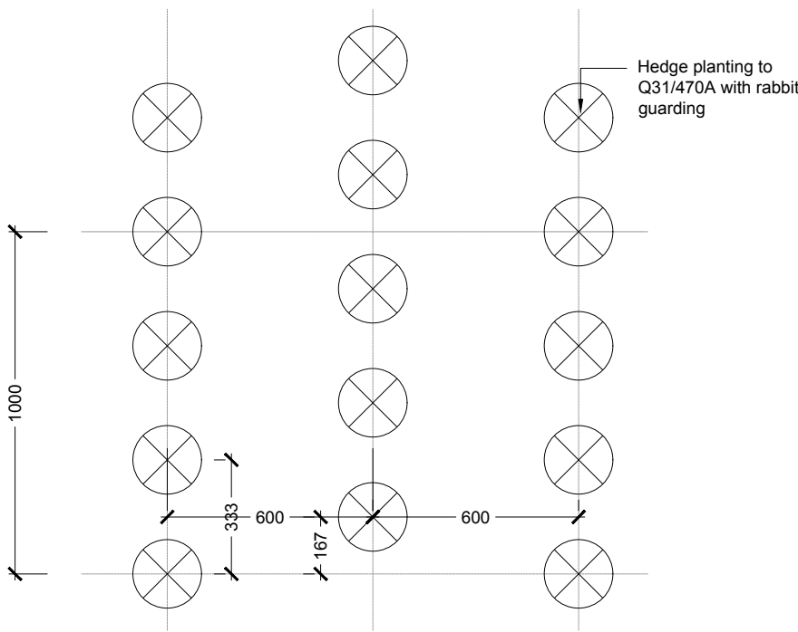
07 TRIPLE STAGGERED HEDGEROW PLAN - REF S2
