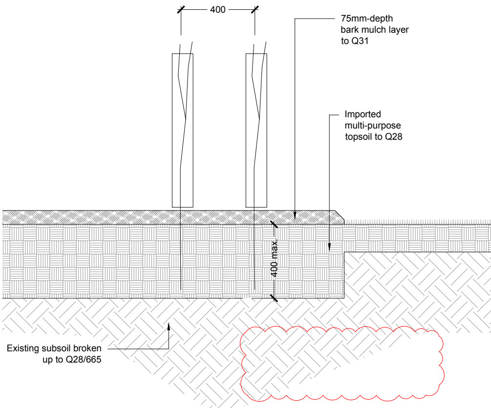
05 TYPICAL DOUBLE STAGGERED HEDGE PLANTING - REF S1/S2
