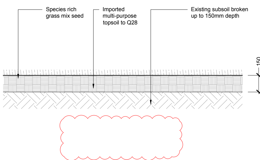
09 SPECIES RICH GRASS MIX SEEDING - REF: M3
