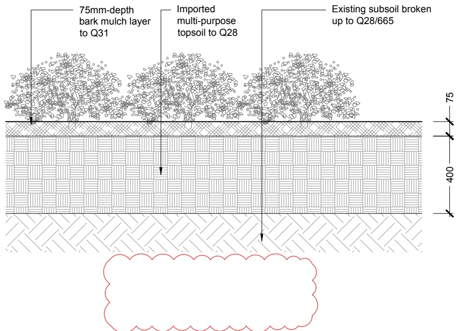
04 SHRUB & HERBACEOUS PLANTING - REF: S3/S4/S5/S6/S7
