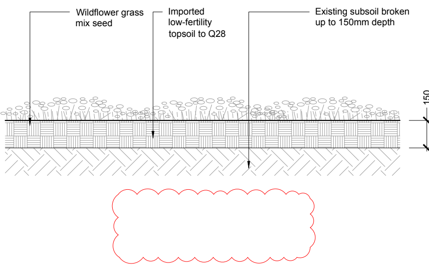
11 WILDFLOWER GRASS MIX SEEDING - REF: M1/M2/M5/M6
