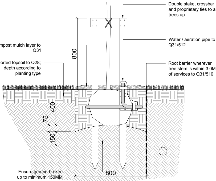
03 TYPICAL HALF STANDARD TREE PIT IN SOFT LANDSCAPE
