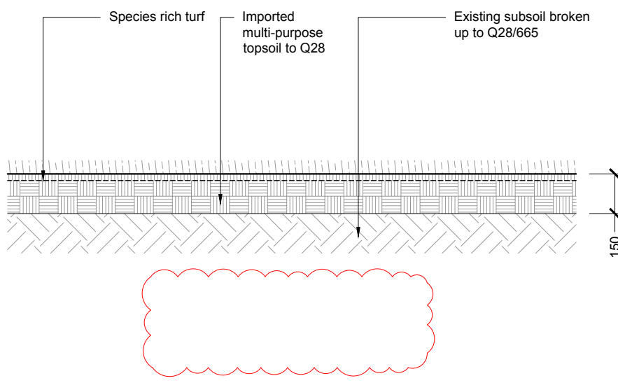
08 SPECIES RICH GRASS TURF - REF: M3
