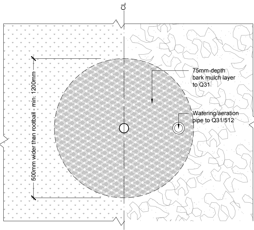
01 TYPICAL EHS/MS TREE PIT IN SOFT LANDSCAPE
