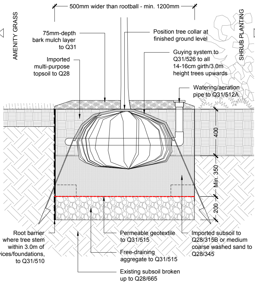
02 TYPICAL EHS/MS TREE PIT IN SOFT LANDSCAPE
