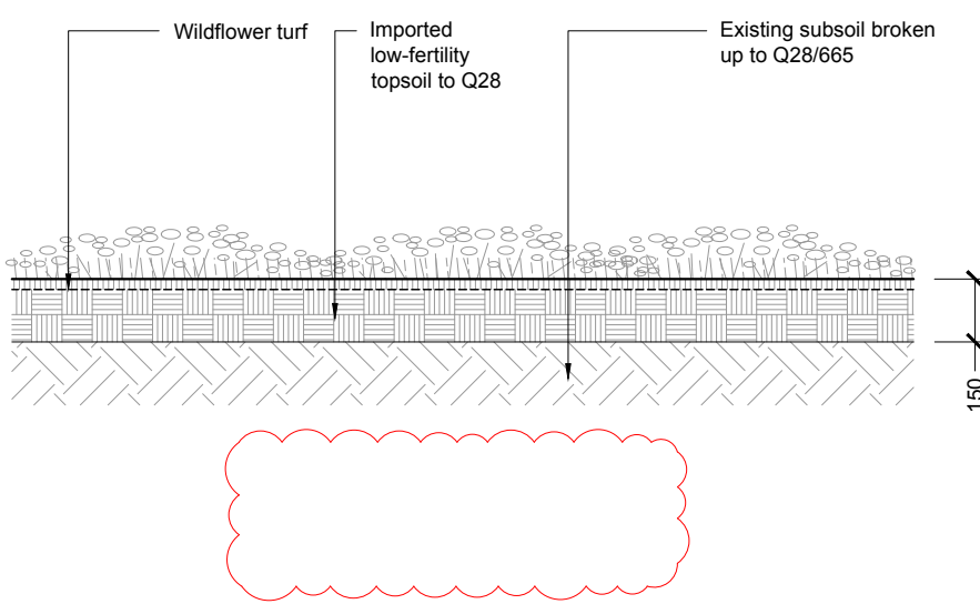
10 WILDFLOWER GRASS TURF - REF: M1/M2/M5
