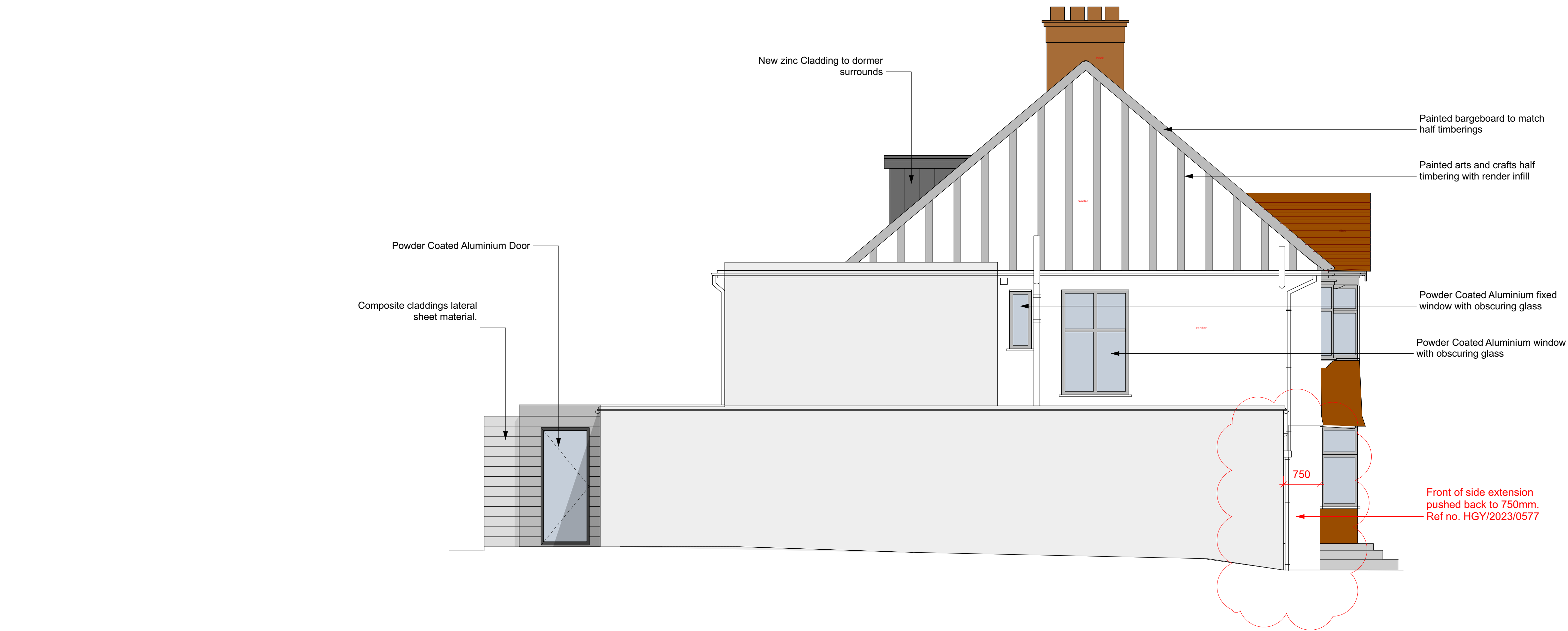
PROPOSED SIDE ELEVATION Scale 1 : 100 @ A3
