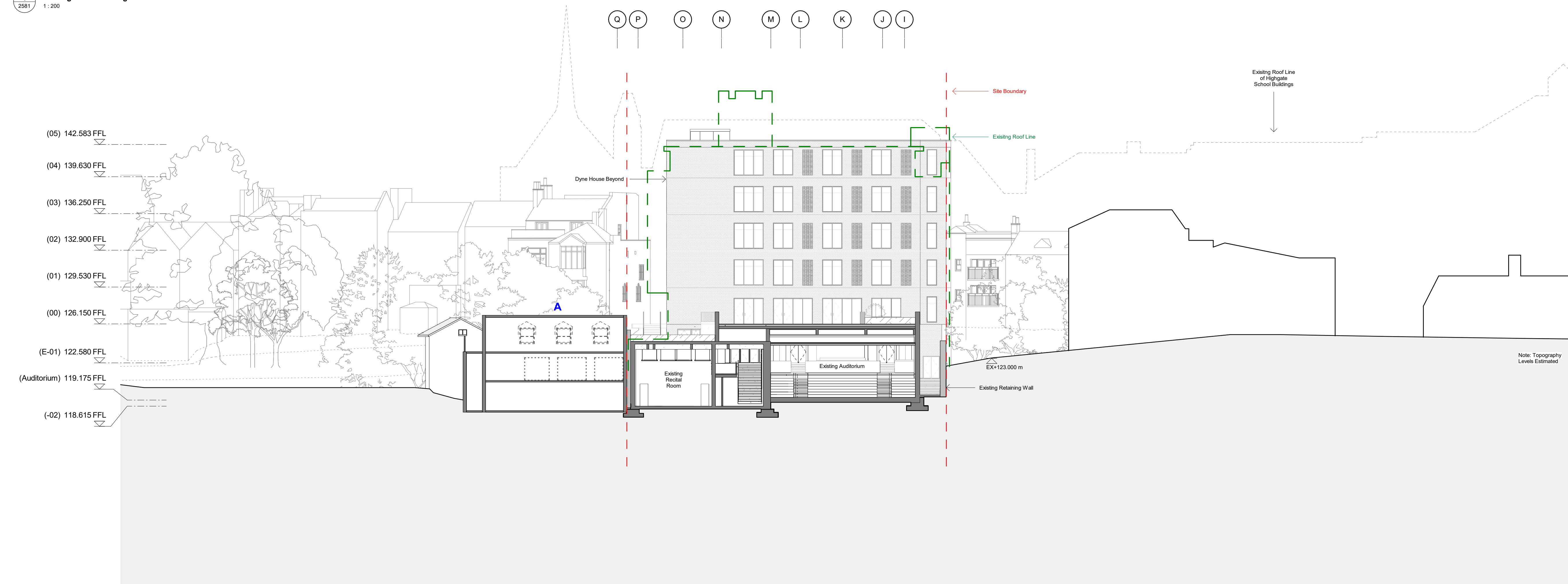
2 2581 Proposed Section through Auditorium - Outline of existing buildings overlaid 1 : 200
