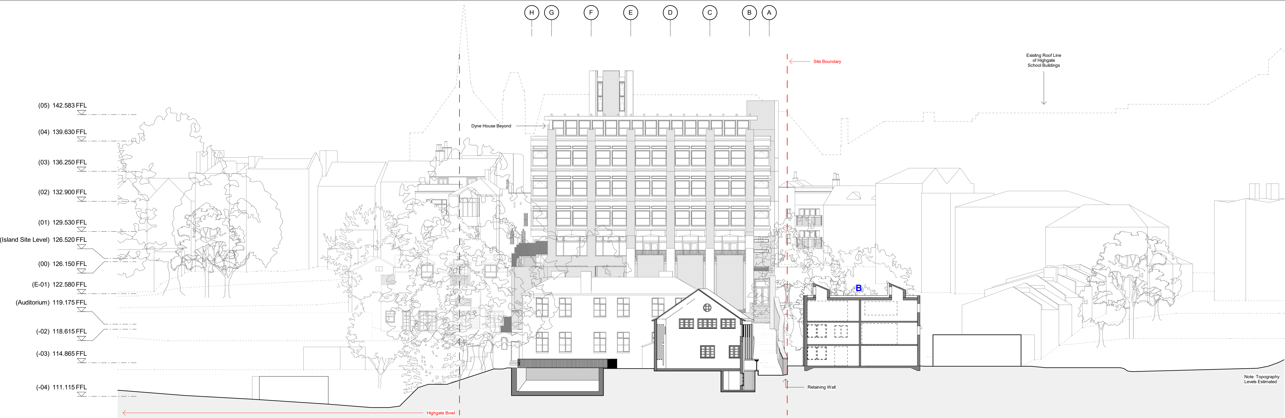
1 Existing Section through Pool + Gym 1 : 200
