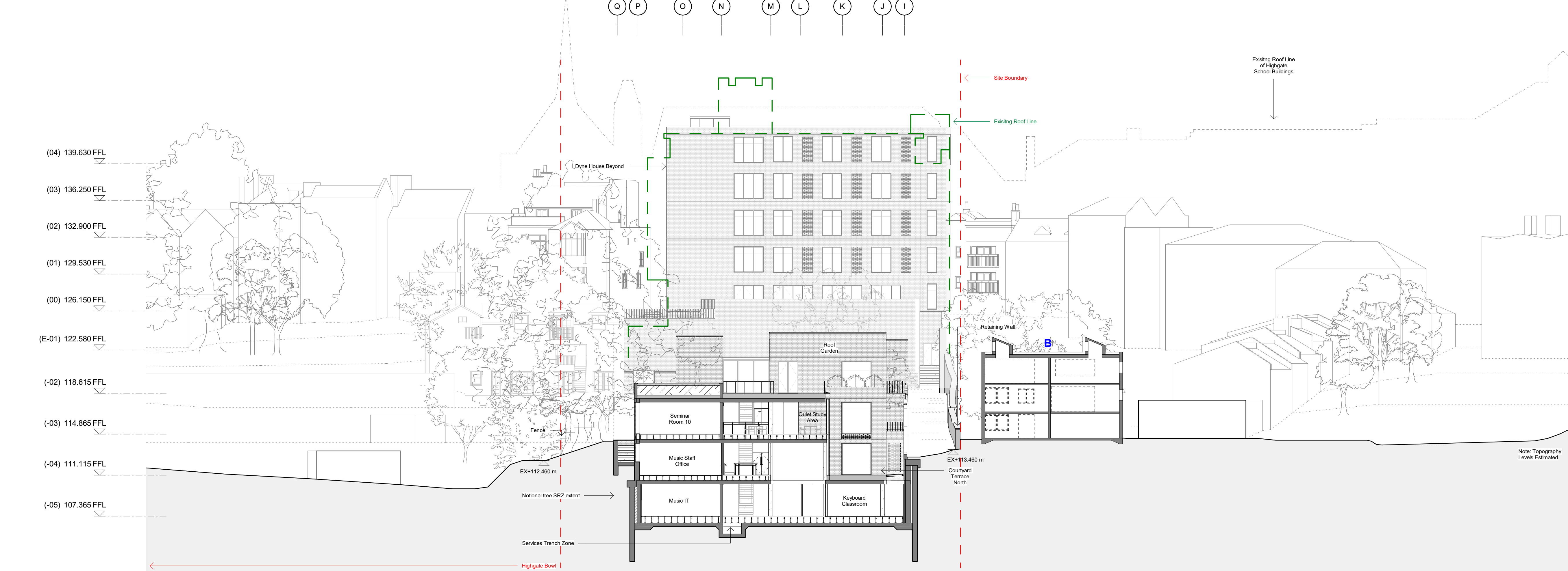
2 Proposed Section through North Courtyard - Outline of existing buildings overlaid 1 : 200
