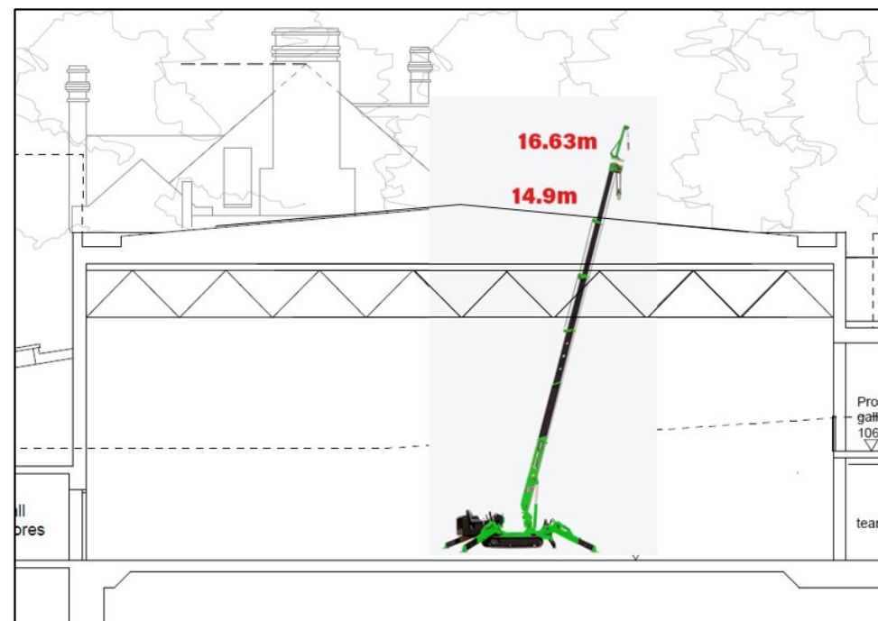
Spider Crane
