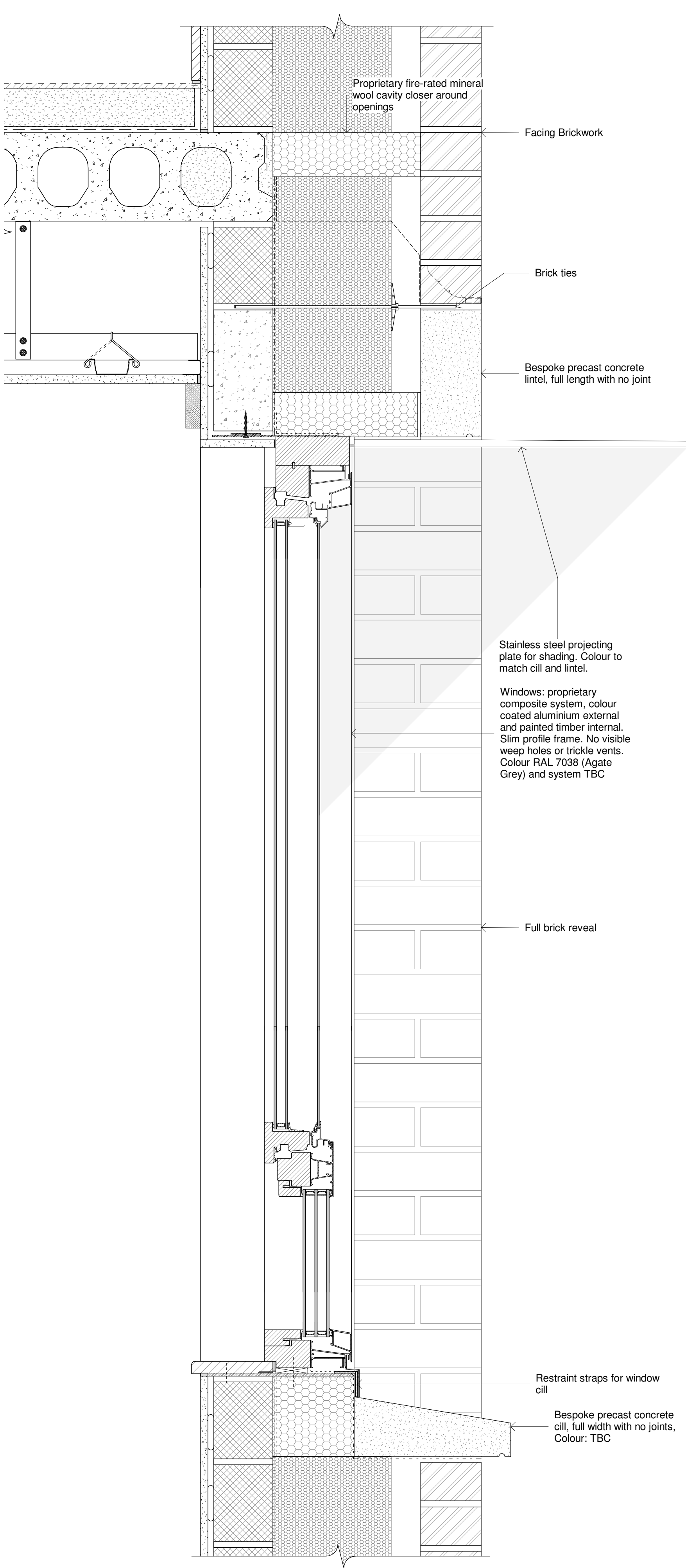
1 Typical window head and cill details
