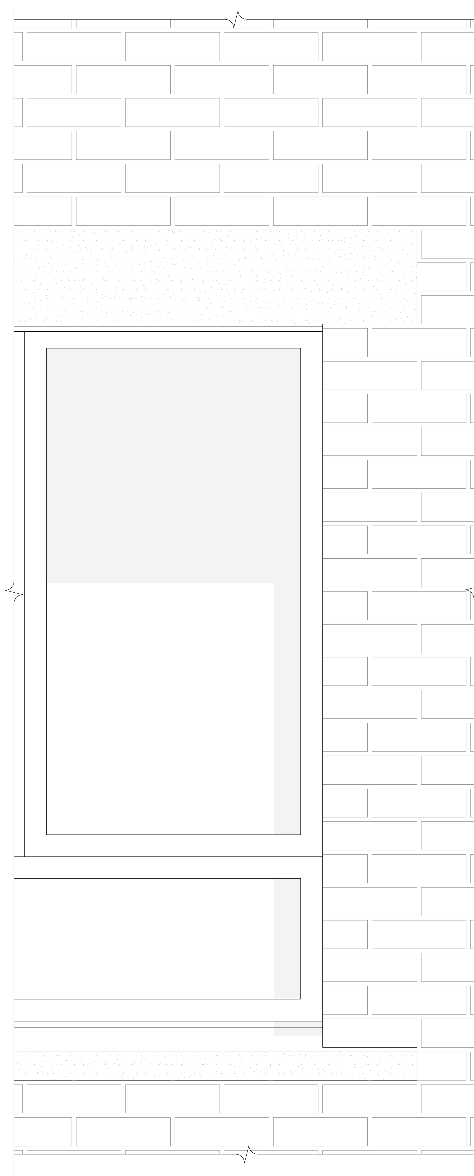
Typical window elevation
