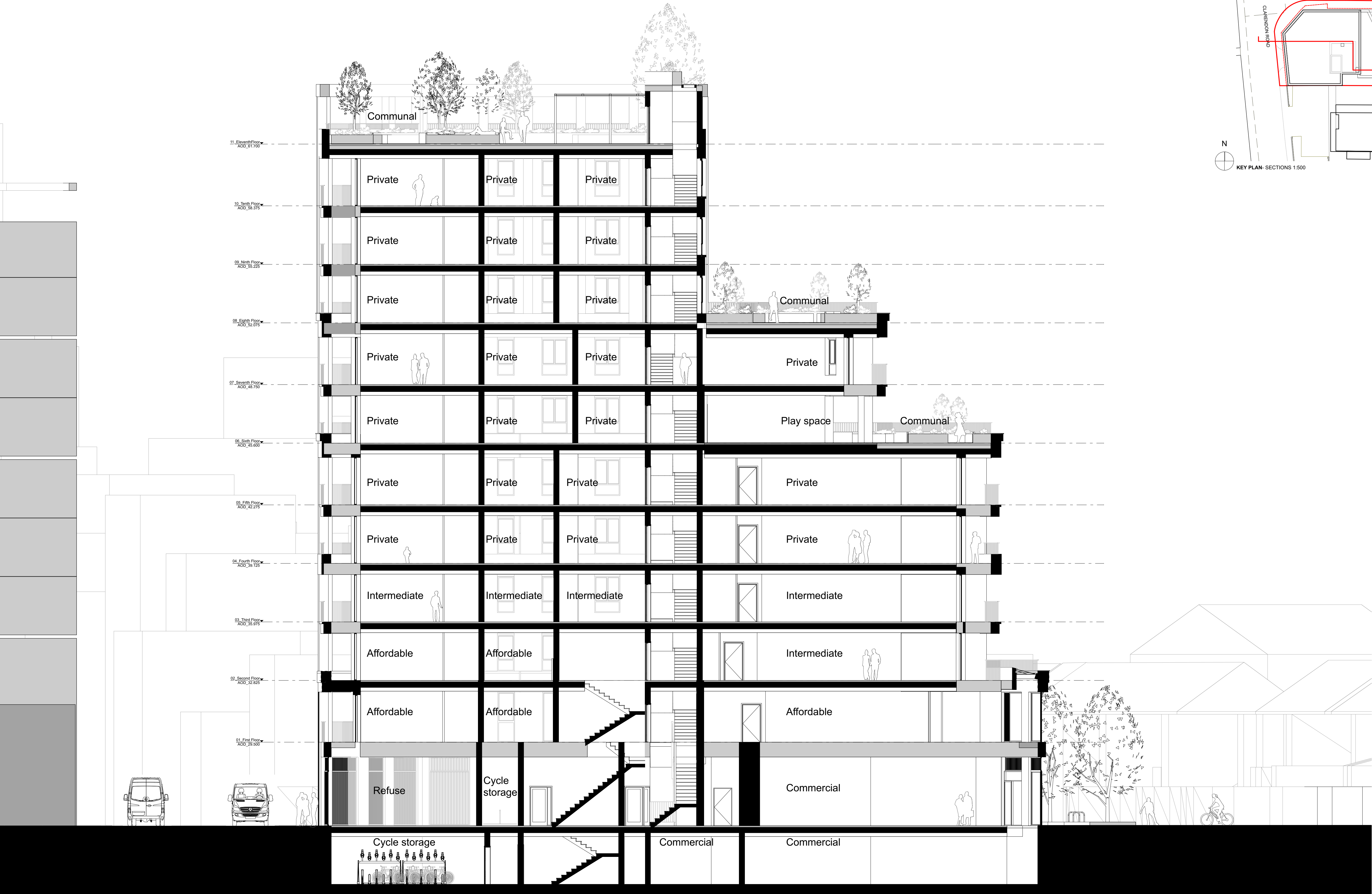
0 6 12 18m B-B' NORTH - SOUTH SECTION
