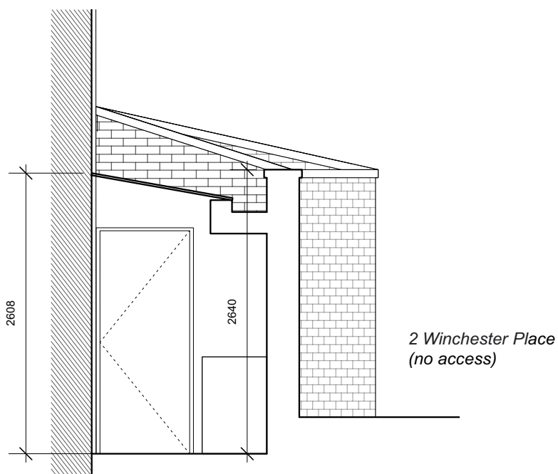
3 Proposed Section CC Scale: 1:50
