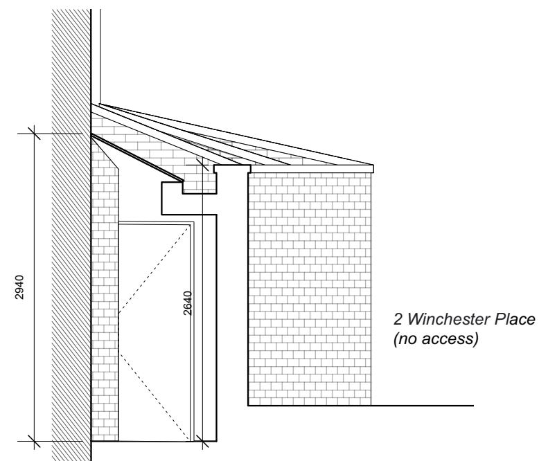
4 Proposed Section BB Scale: 1:50
