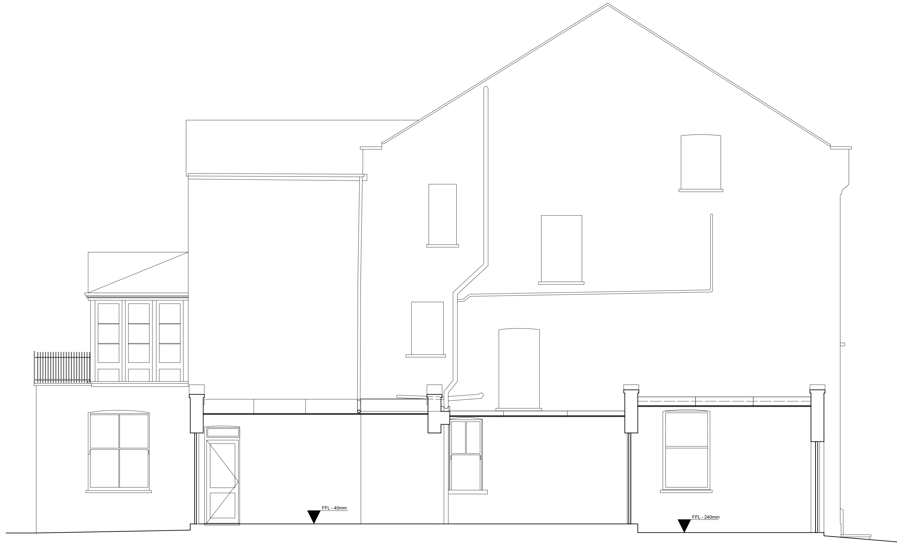
1 Proposed Section AA Scale: 1:50
