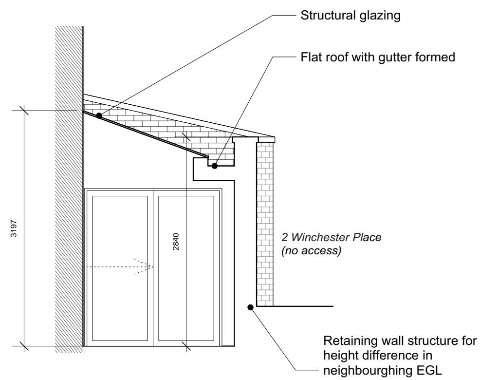
2 Proposed Section DD Scale: 1:50
