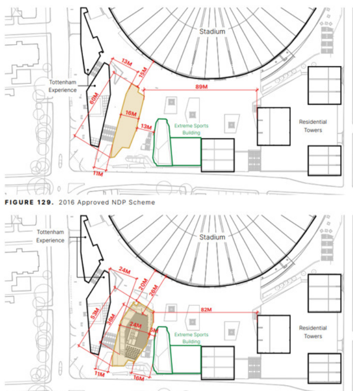
Figure 8: separation distances
